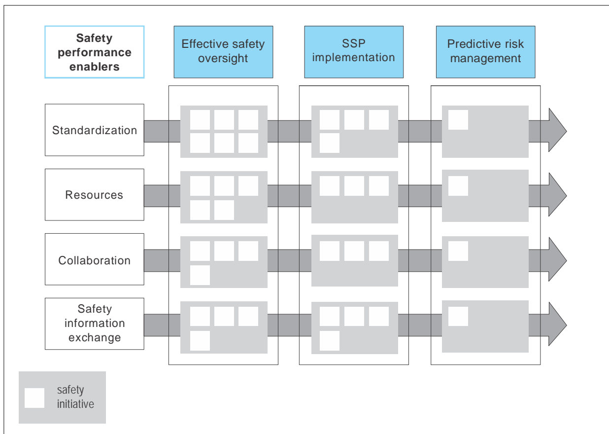
Figure 4-1. GASP framework
