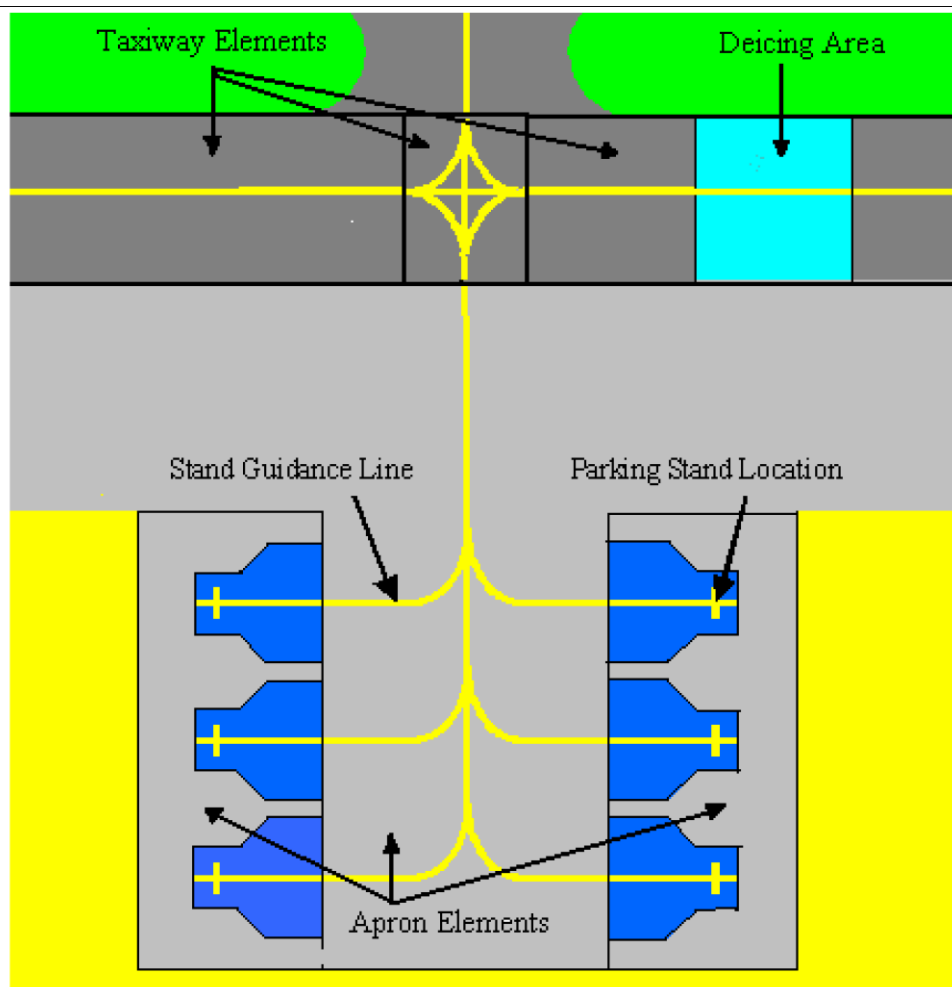
Figure 33: Apron elements
