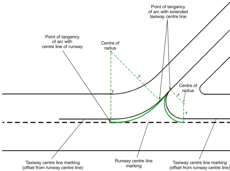
Figure 17: Sample detail for Taxiway on Runway Marking
