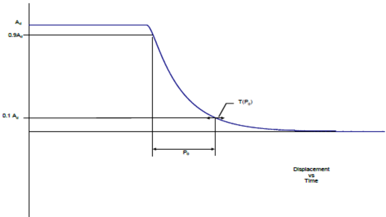
Figure 2: Critically damped step response
