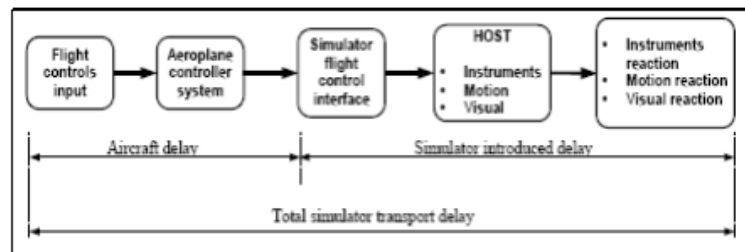
Figure 1: Transport delay for simulation of classic non-computer-controlled aircraft
