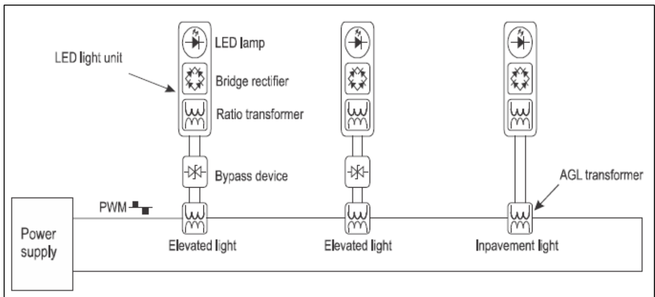
Figure 11-7. Use of a power supply to produce PWM output
