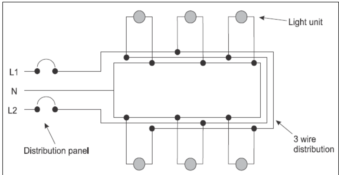
Figure 4-2. Parallel circuit
