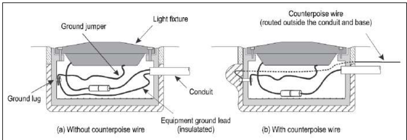
Figure 12-22. Shallow base installation
