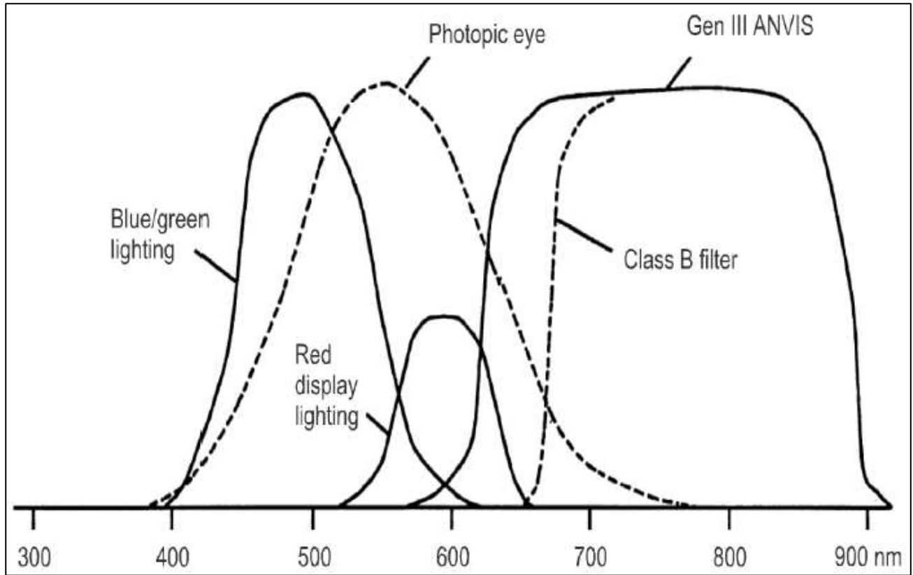
Figure 11-16. Class B filter allows blue, green, yellow and red cockpit lighting (source: Dennis L. Schmickley, Boeing Helicopter Co.)
