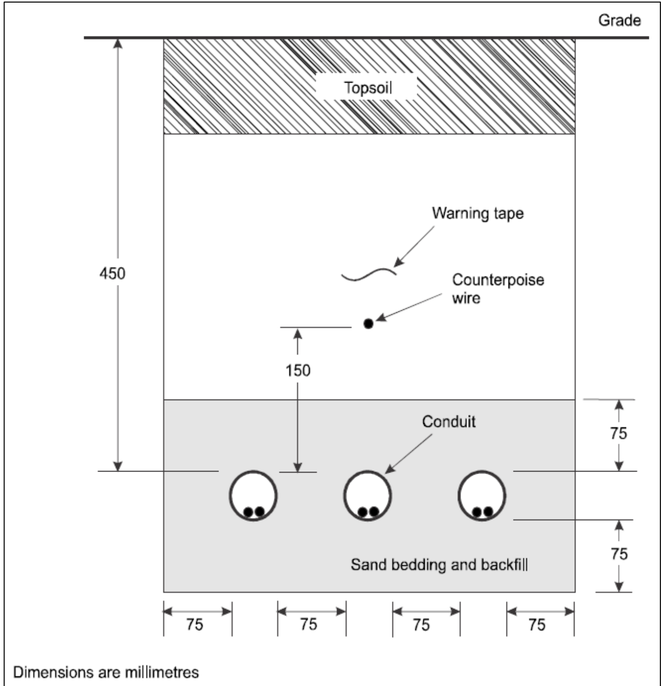
Figure 12-10. Duct/conduit without concrete encasement
