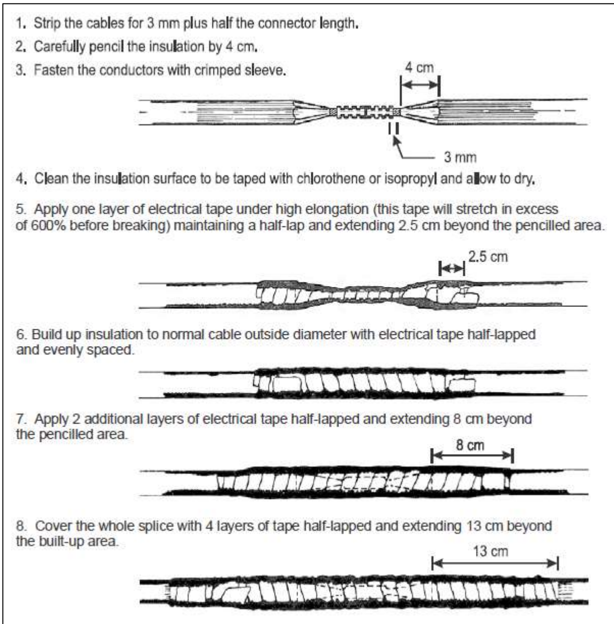
Figure 13-3. Taped splice – Typical (refer to the manufacturer’s instructions)
