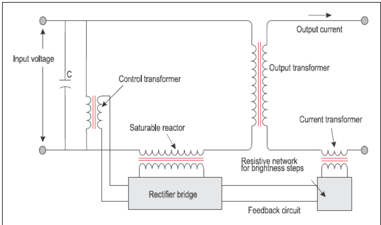
Figure 6-3. Saturable reactor regulator
