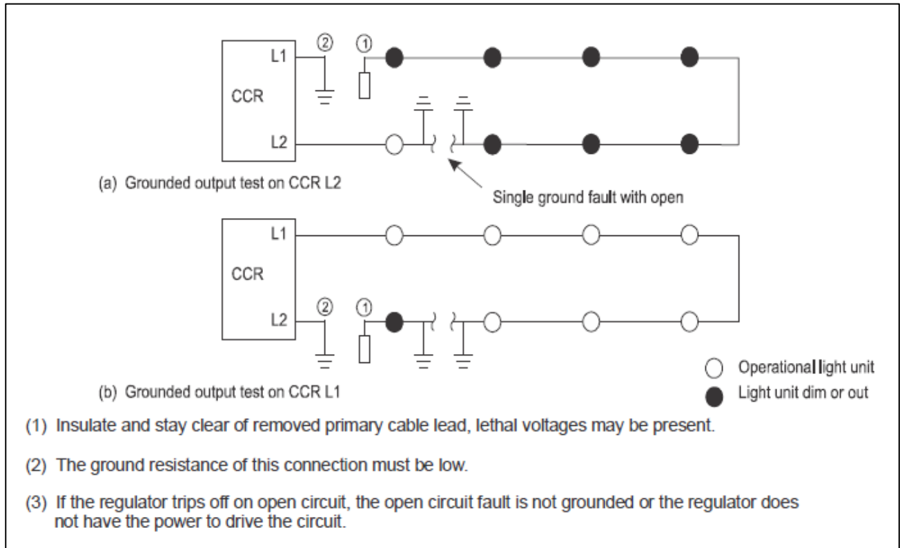
Figure 15-10. Grounded output test
