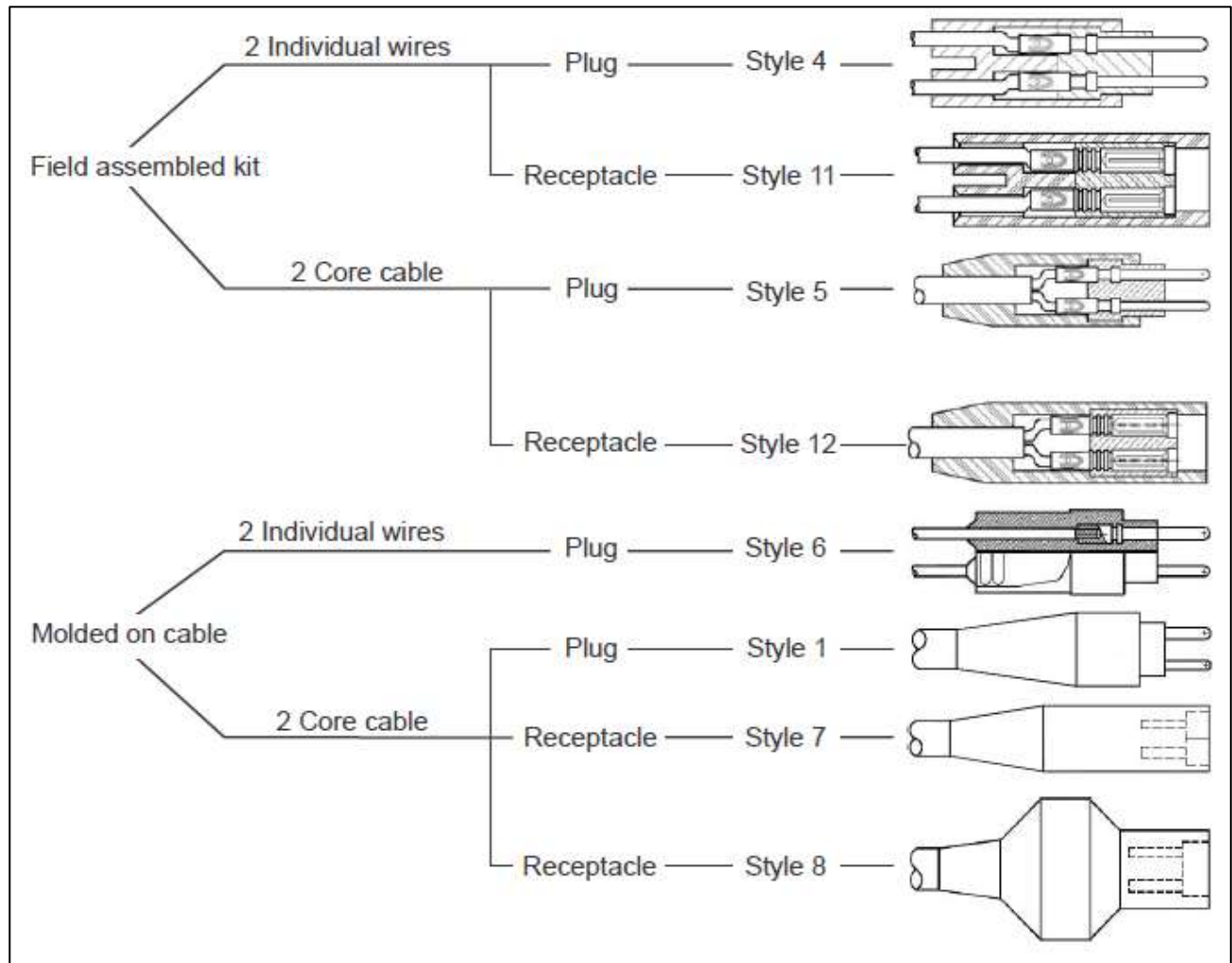
Figure 13-6. Secondary connectors
