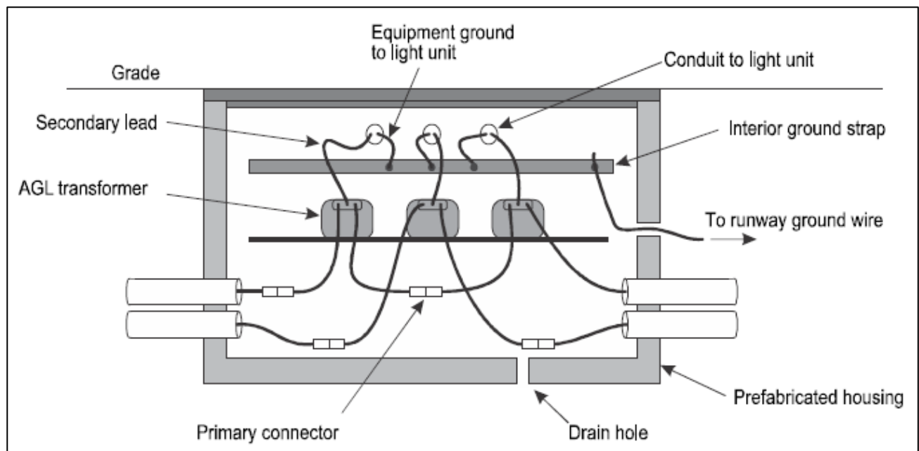
Figure 12-21. Multiple transformers in a prefabricated housing
