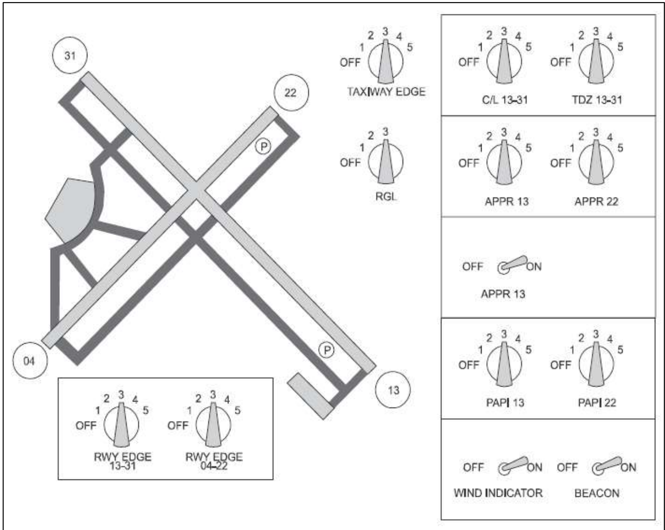
Figure 9-5. Mimic diagram with physical controls
