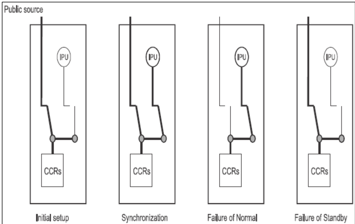
Figure 2-3. Synchronization of sources
