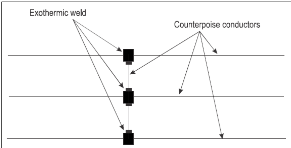
Figure 12-9. Counterpoise interconnections
