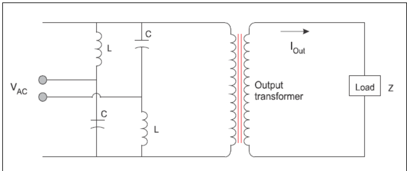
Figure 6-2. Resonant network regulators
