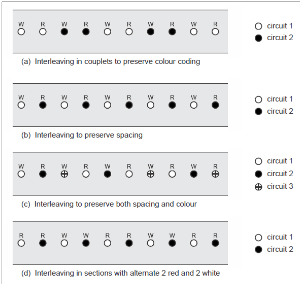
Figure 5-4. Interleaving of colour coded lights
