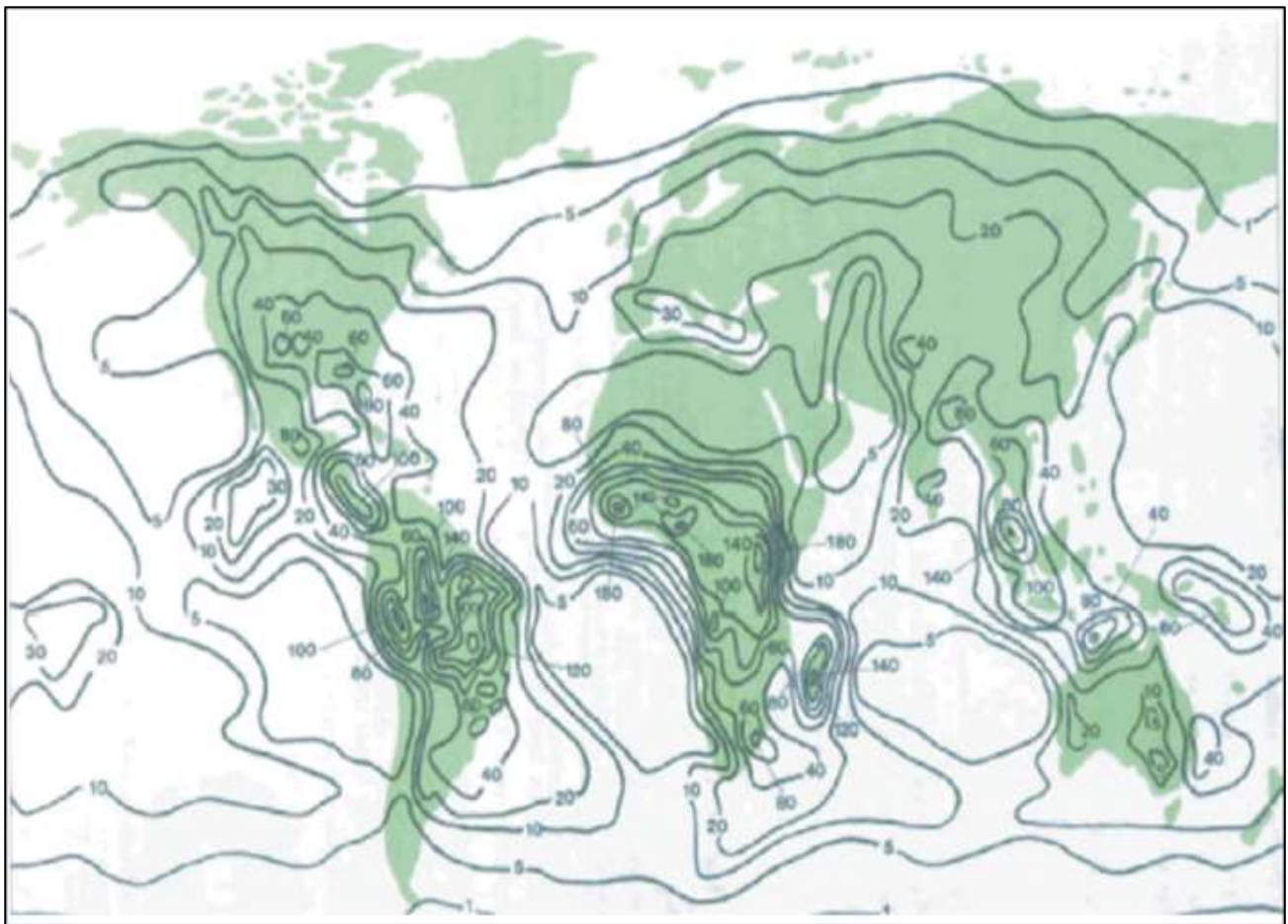
Figure 3-2. Iso-Keraunic lines (adapted from WMO publication 21 (1956))
