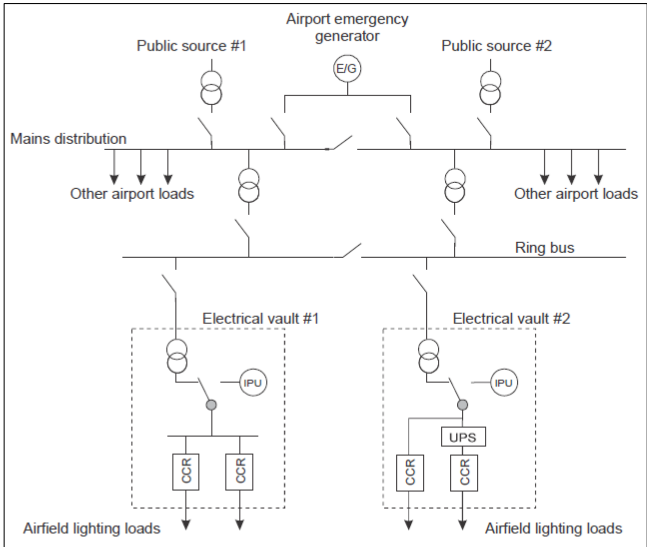
Figure 3-1. Power schematic
