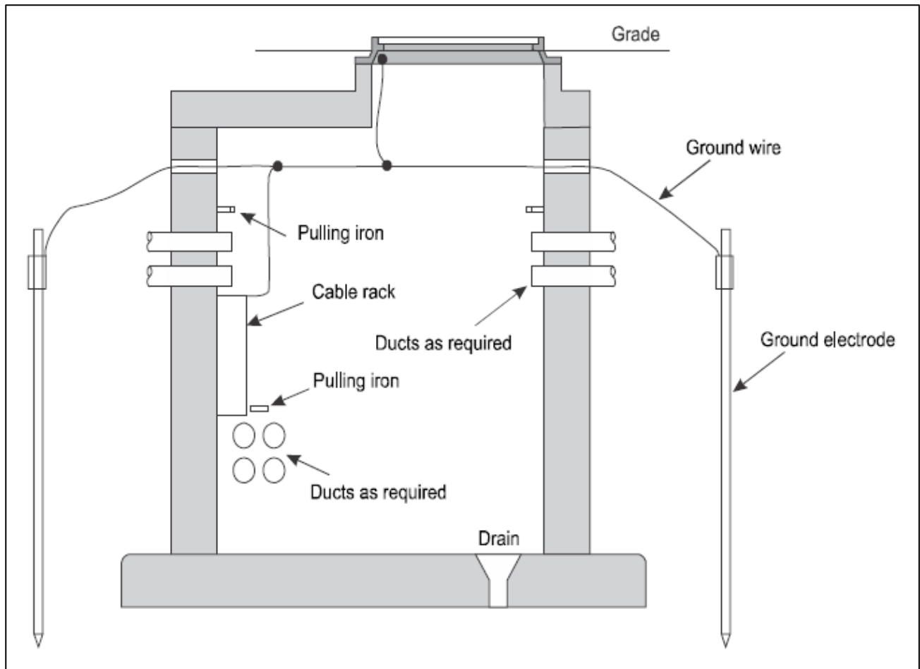
Figure 12-13. Manhole
