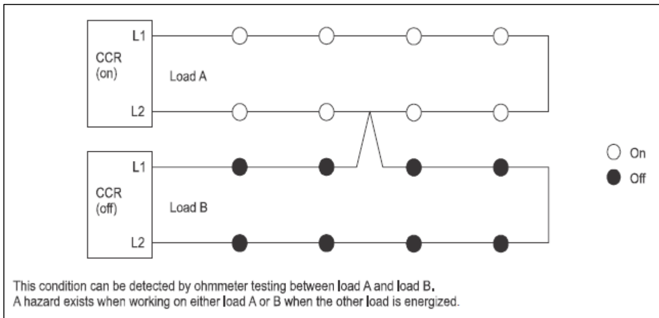
Figure 15-6. Single load-to-load fault
