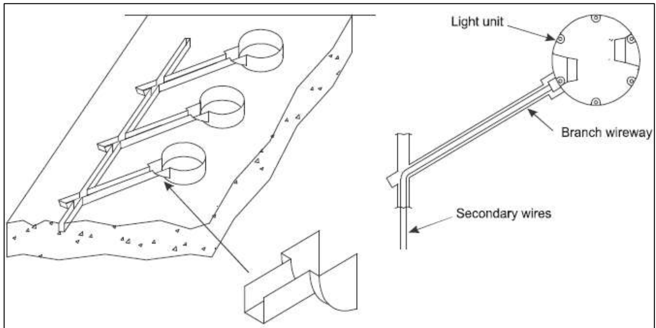
Figure 12-14. Saw kerf detail
