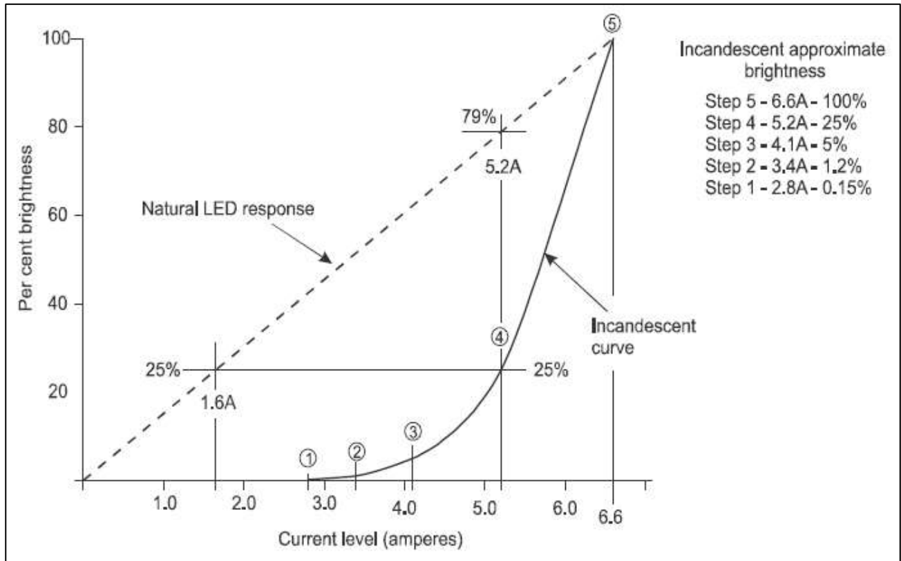
Figure 11-9. LED and incandescent lighting response curves
