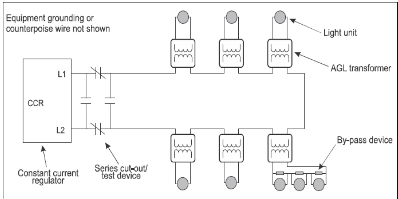
Figure 4-1. Series lighting circuit
