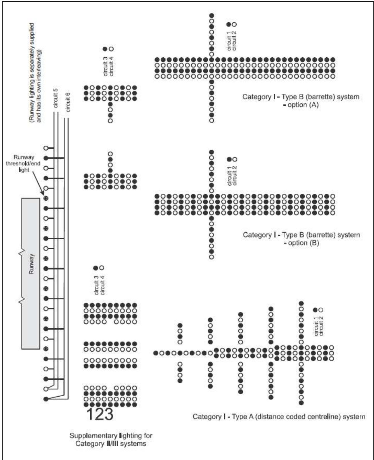
Figure 5-3. Precision approach lighting system interleaving
