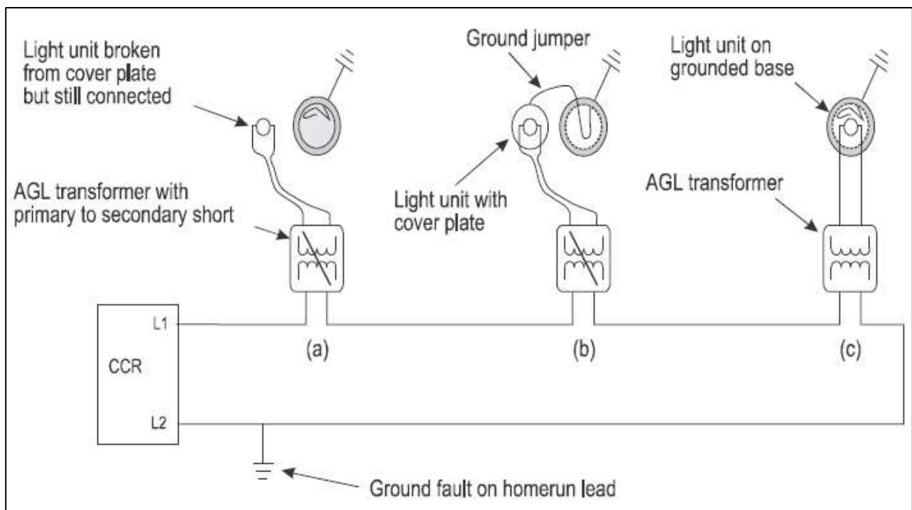
Figure 15-1. Dangerous isolation transformer/circuit ground faults
