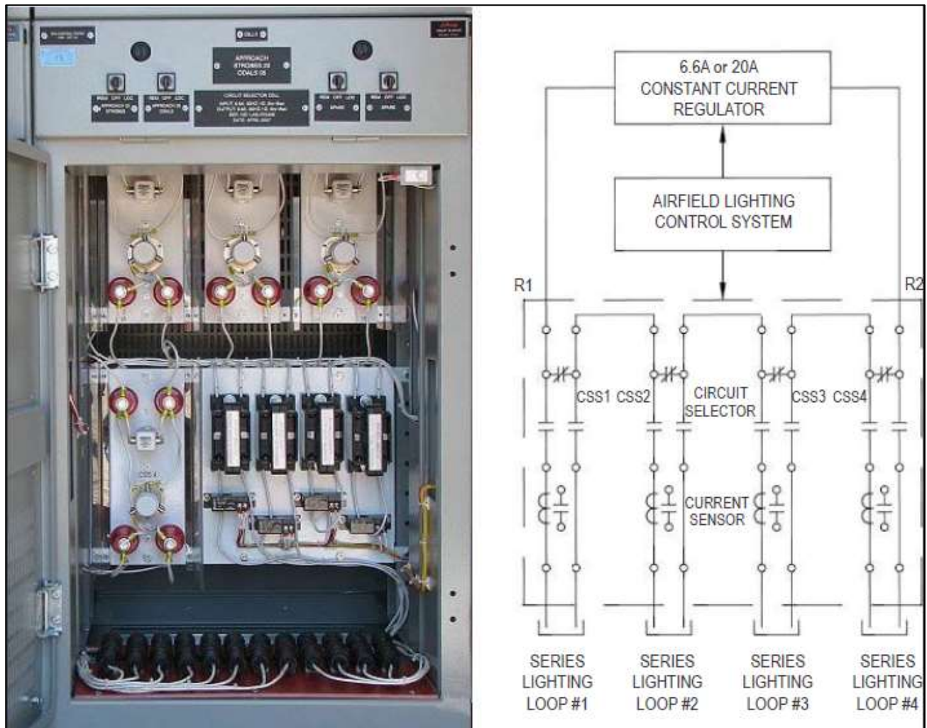
Figure 9-9. Selector relay cabinet (source: Liberty Airfield Lighting)
