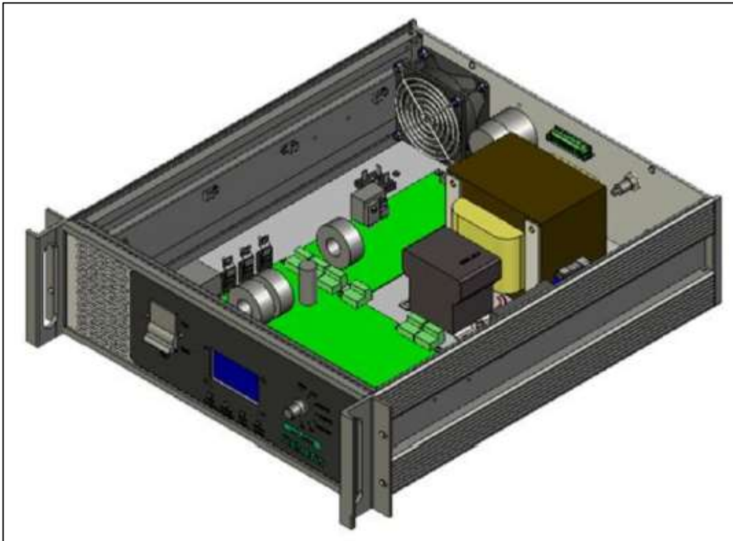
Figure 11-8. PWM power supply (source: ADB Airfield Solutions)
