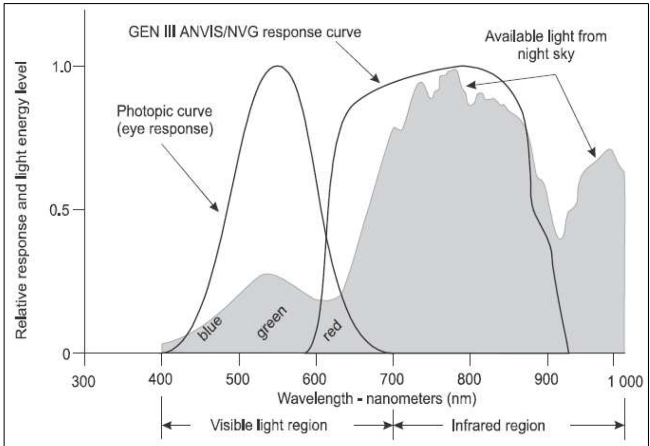
Figure 11-14. Response of GEN III ANVIS/NVG night vision goggles with respect to night sky radiation (source: Gamma Scientific)
