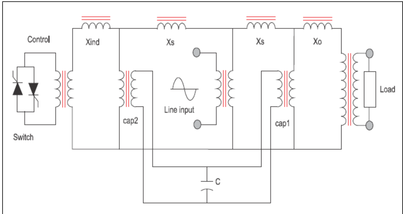
Figure 6-5. Ferroresonant regulator
