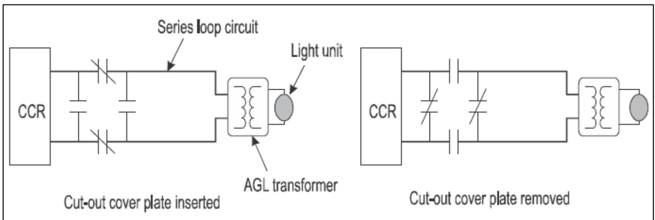
Figure 4-4. Series cut-out device (diagram)
