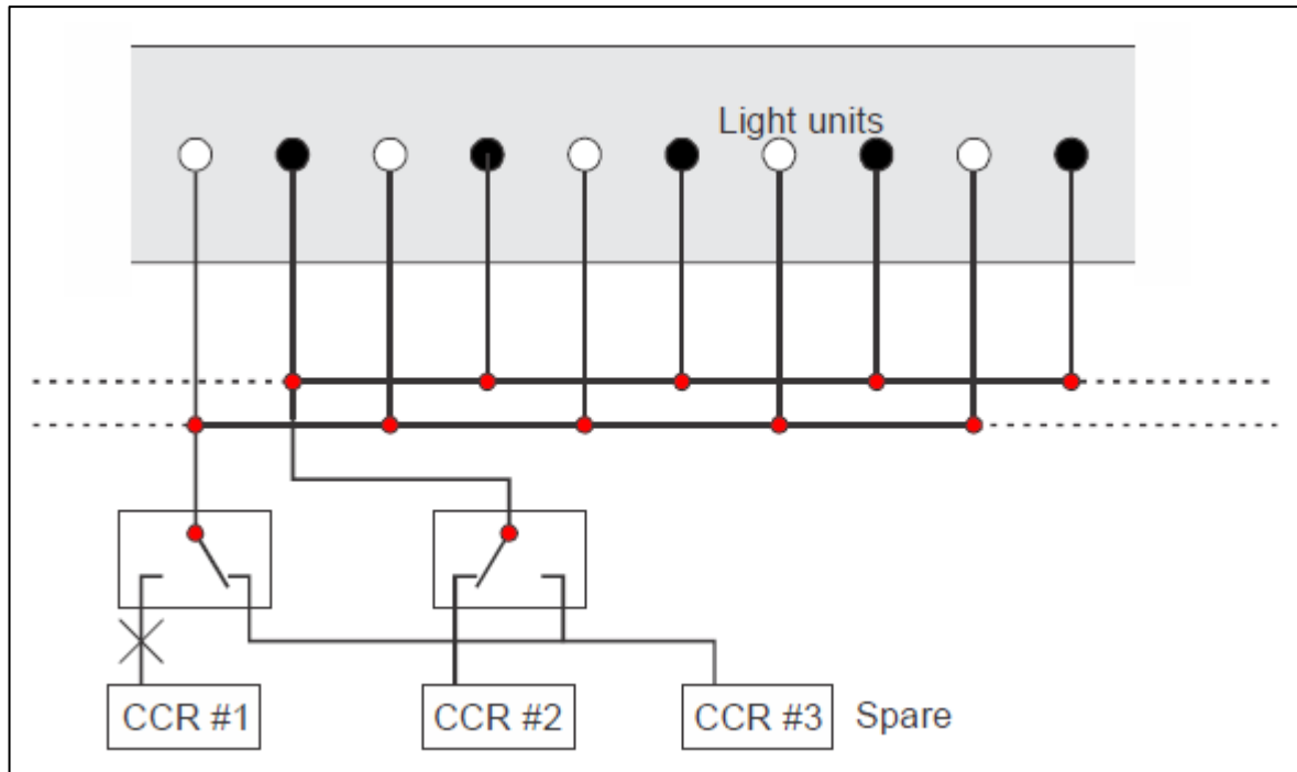
Figure 5-2. Use of spare regulator
