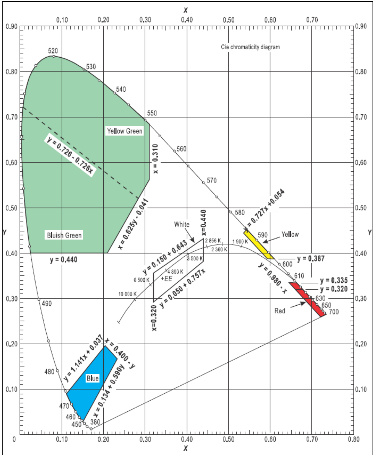
Figure 11-3. Chromaticity boundaries for solid state colours
