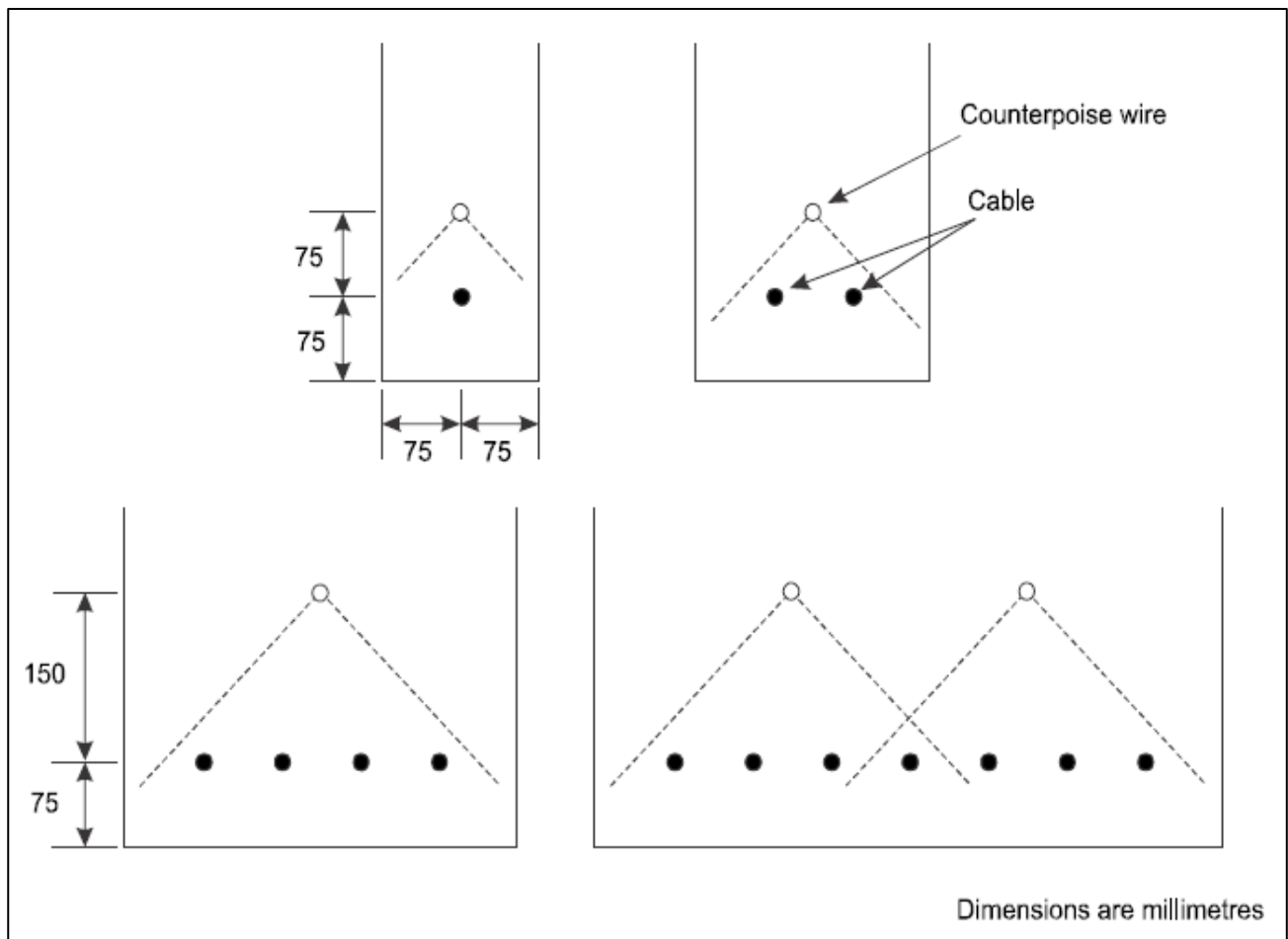
Figure 12-5. Placement of counterpoise wires
