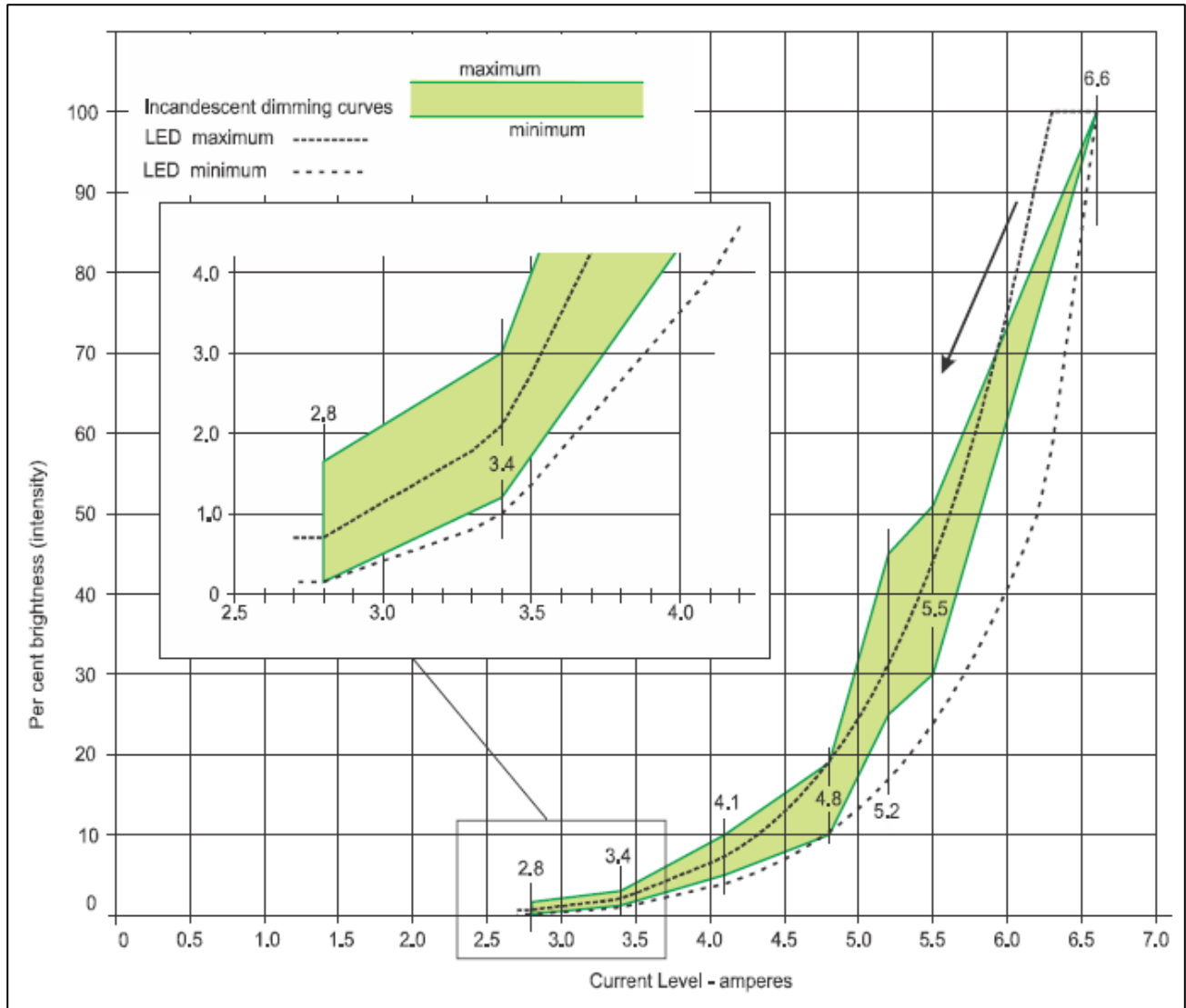
Figure 11-10. Dimming curves, white light
