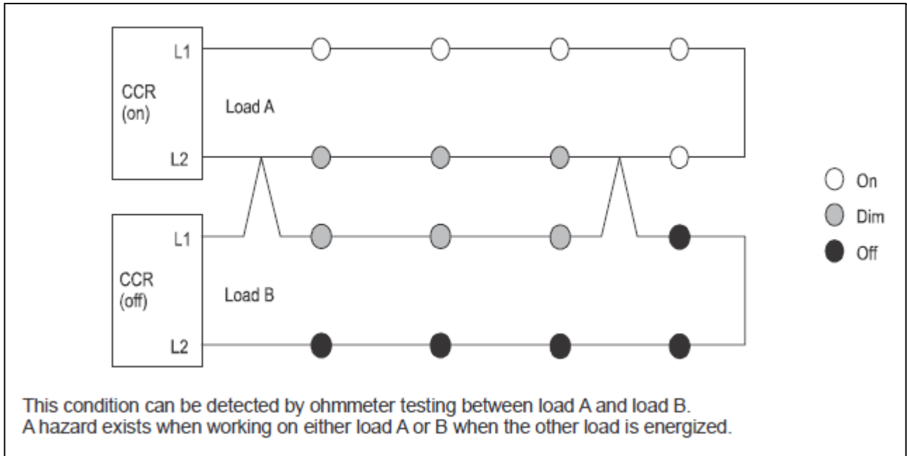
Figure 15-7. Two load-to-load shorts
