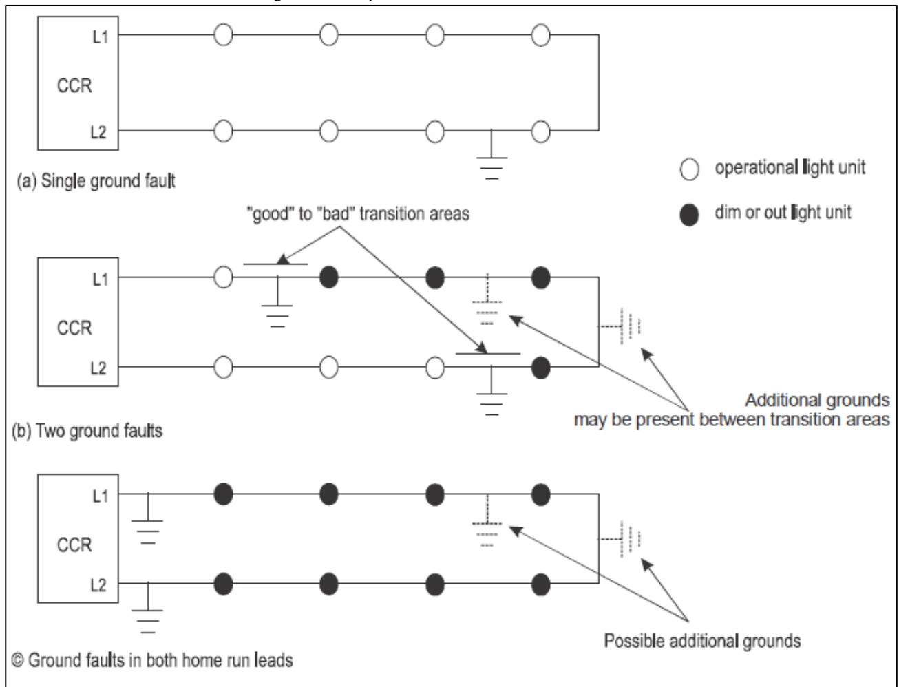
Figure 15-2. Typical ground faults
