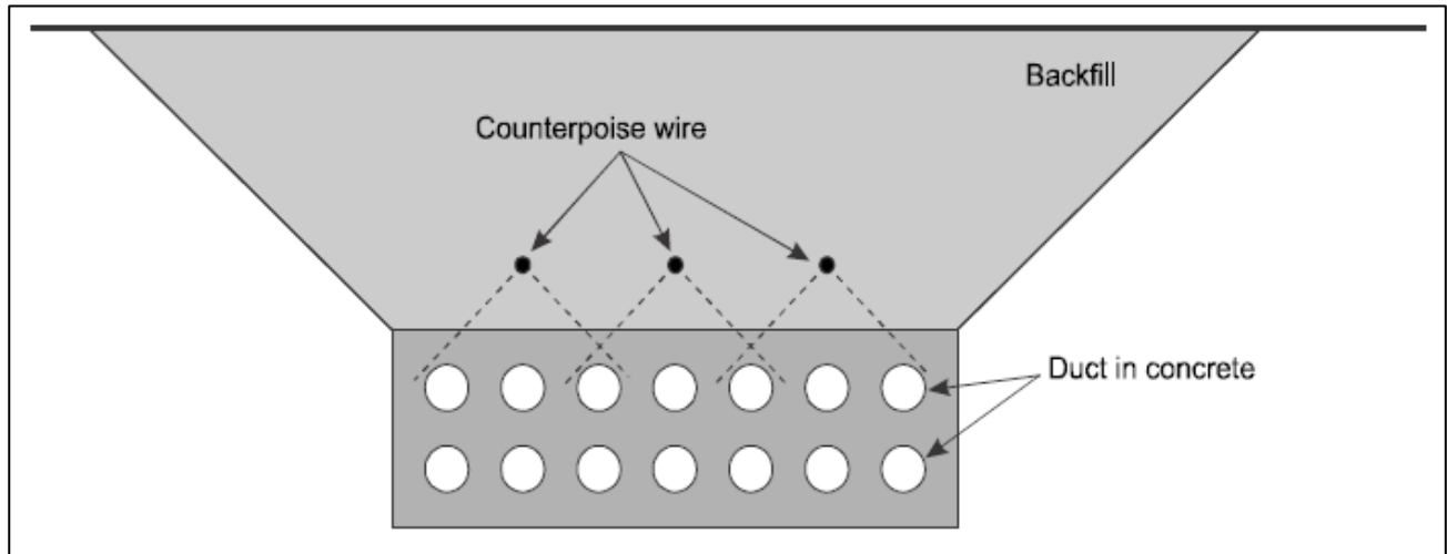
Figure 12-12. Counterpoise above multiple ducts
