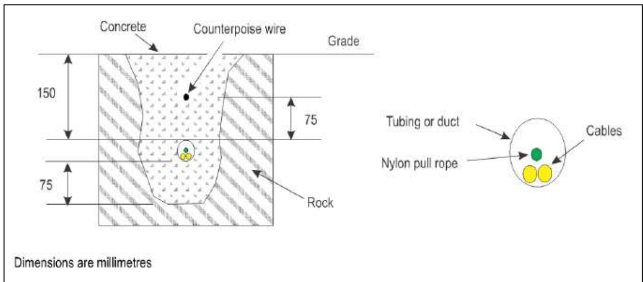
Figure 12-7. Cable/counterpoise lateral spacing
