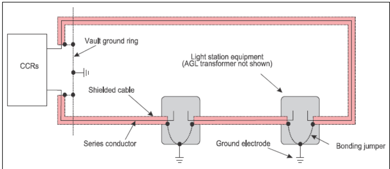
Figure 12-3. Countinuity bonding of shielded cablr
