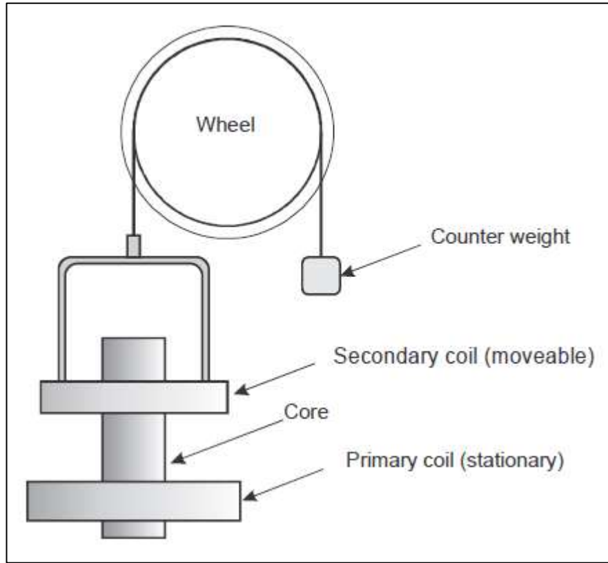
Figure 6-1. Moving coil regulators
