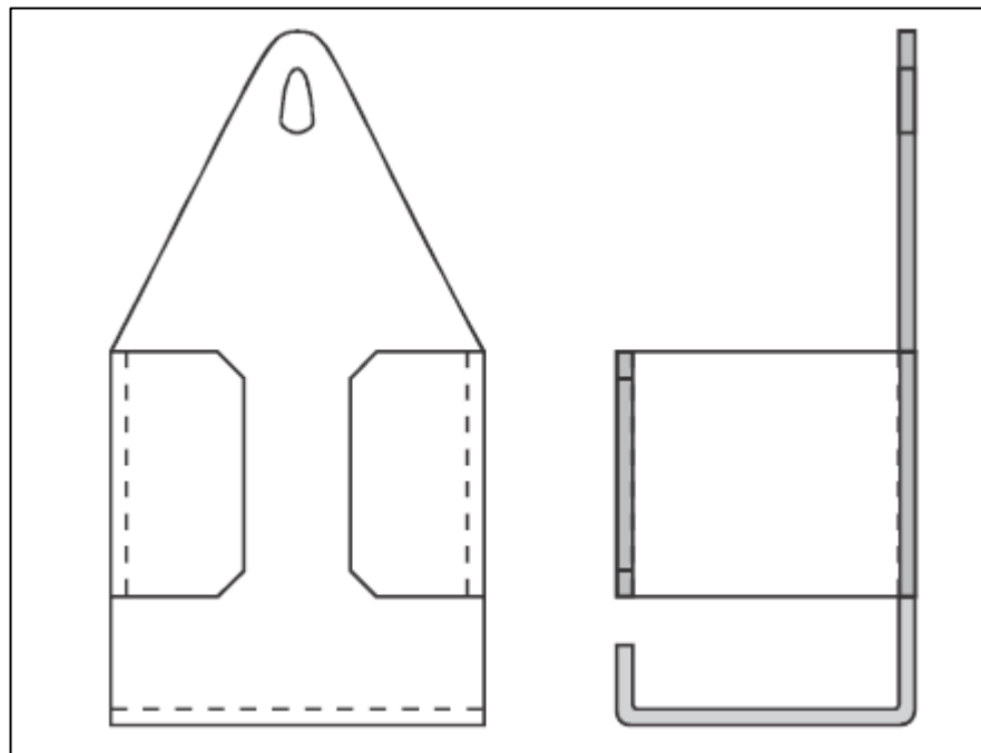
Figure 8-3. Transformer hanger
