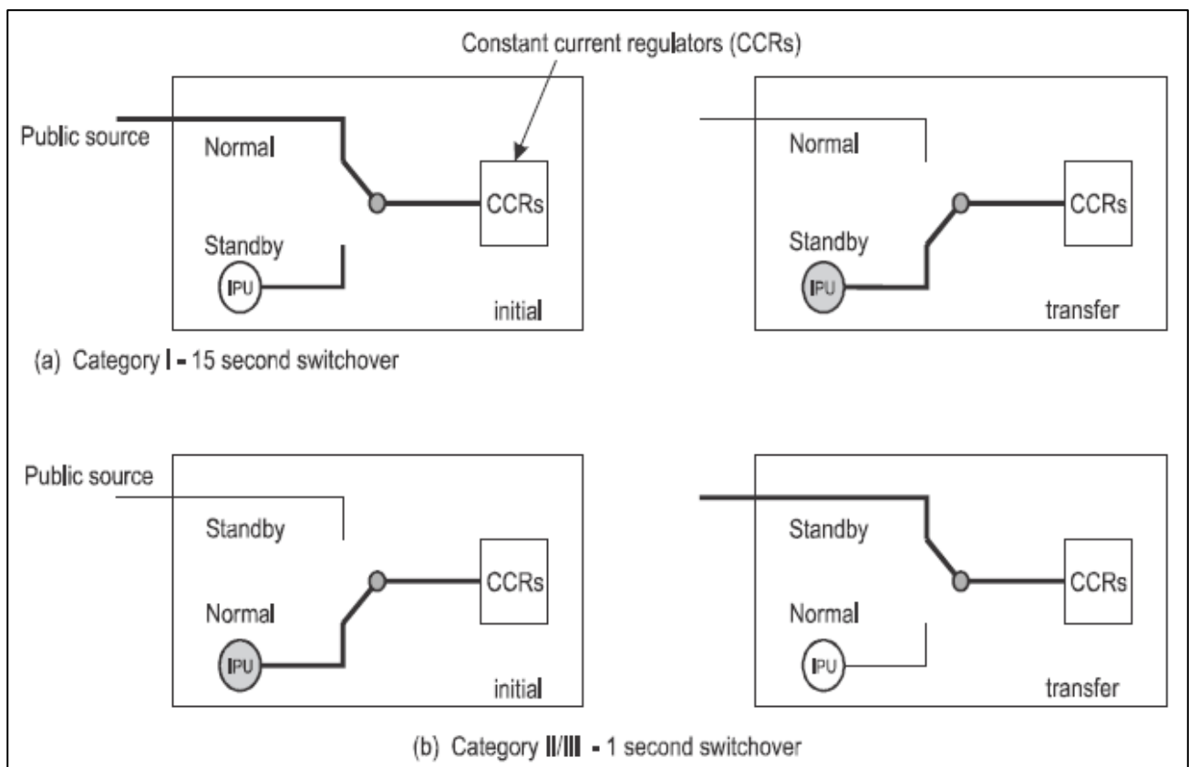
Figure 2-2. Normal and standby power supply
