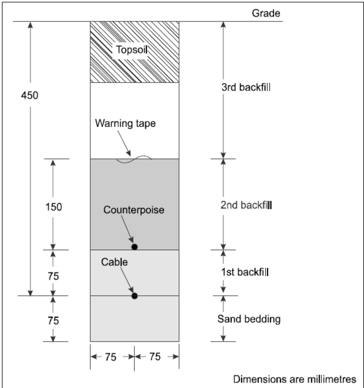
Figure 12-4. Direct burial of cable in trench
