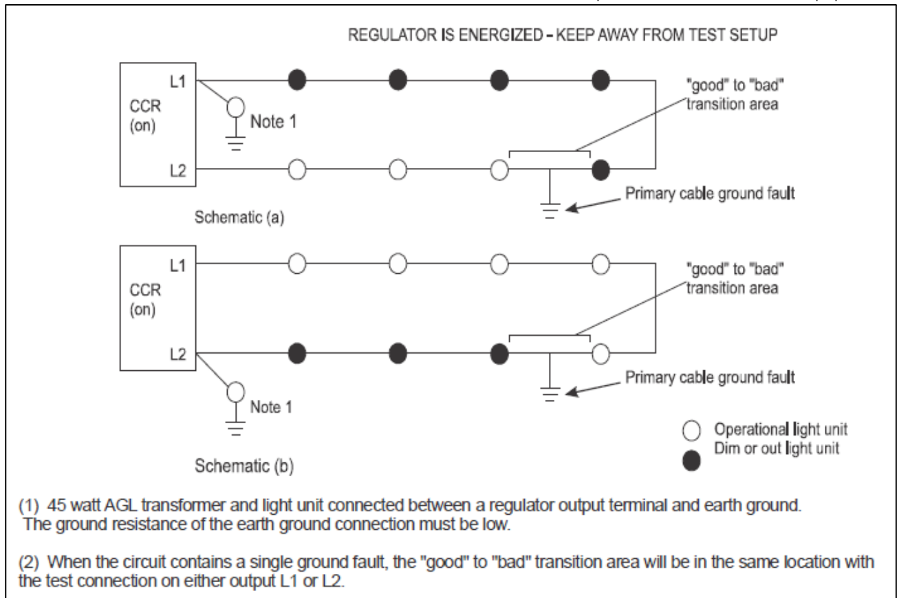
Figure 15-8. Intentional ground test
