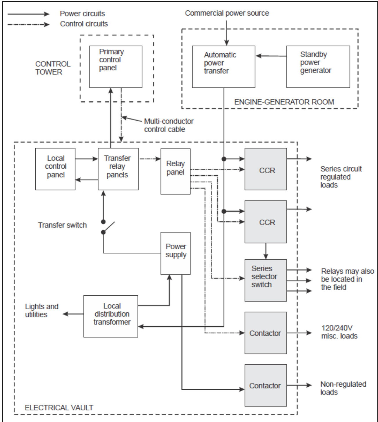
Figure 9-3. Traditional control/monitoring system
