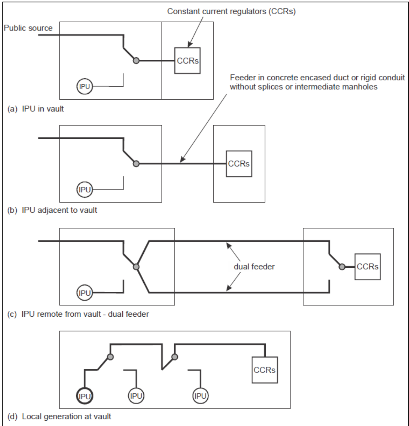
Figure 2-10. IPU configurations
