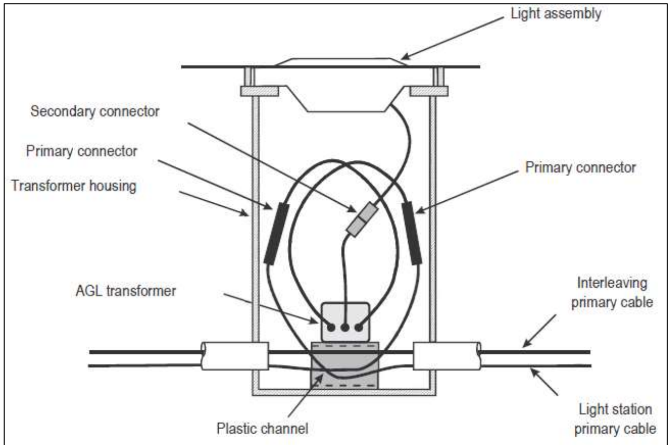
Figure 8-2. Use of plastic channel in housing
