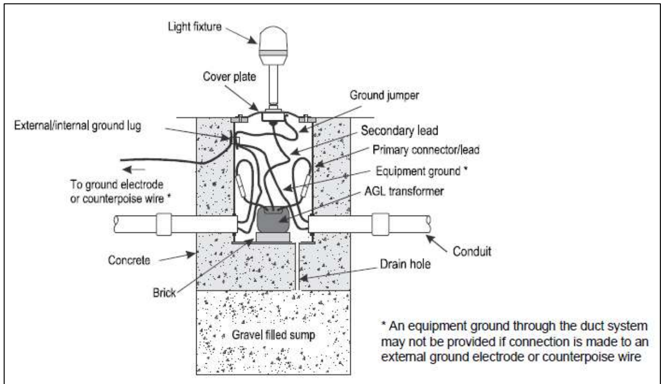
Figure 12-20. Light unit on transformer housing
