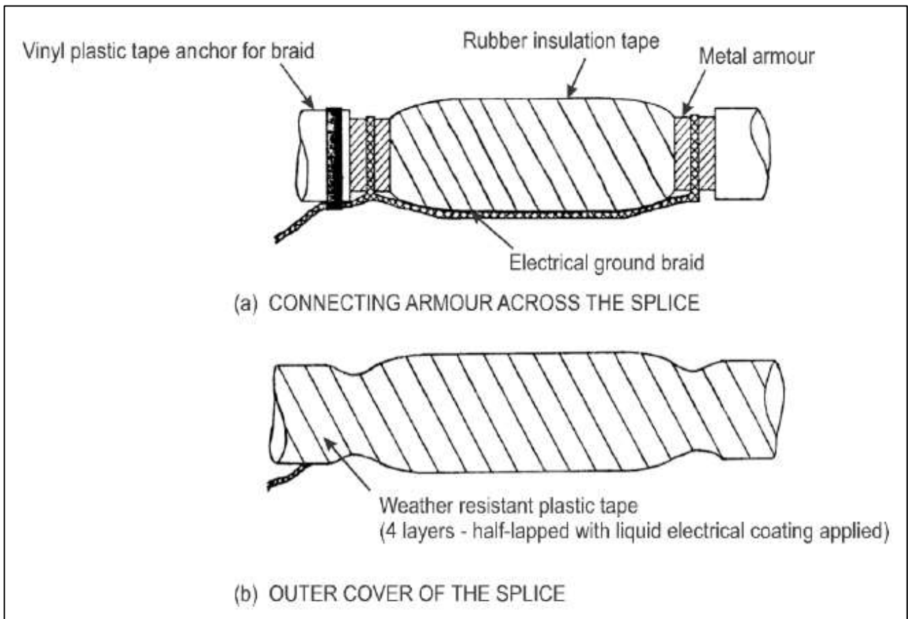
Figure 13-4. Taped splice for metal-armoured cable
