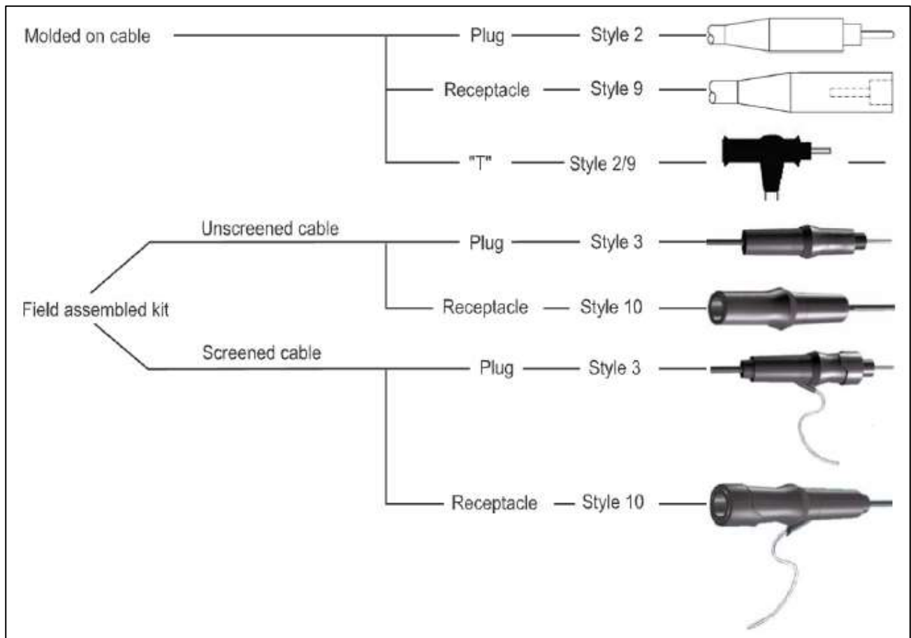
Figure 13-5. Primary connectors
