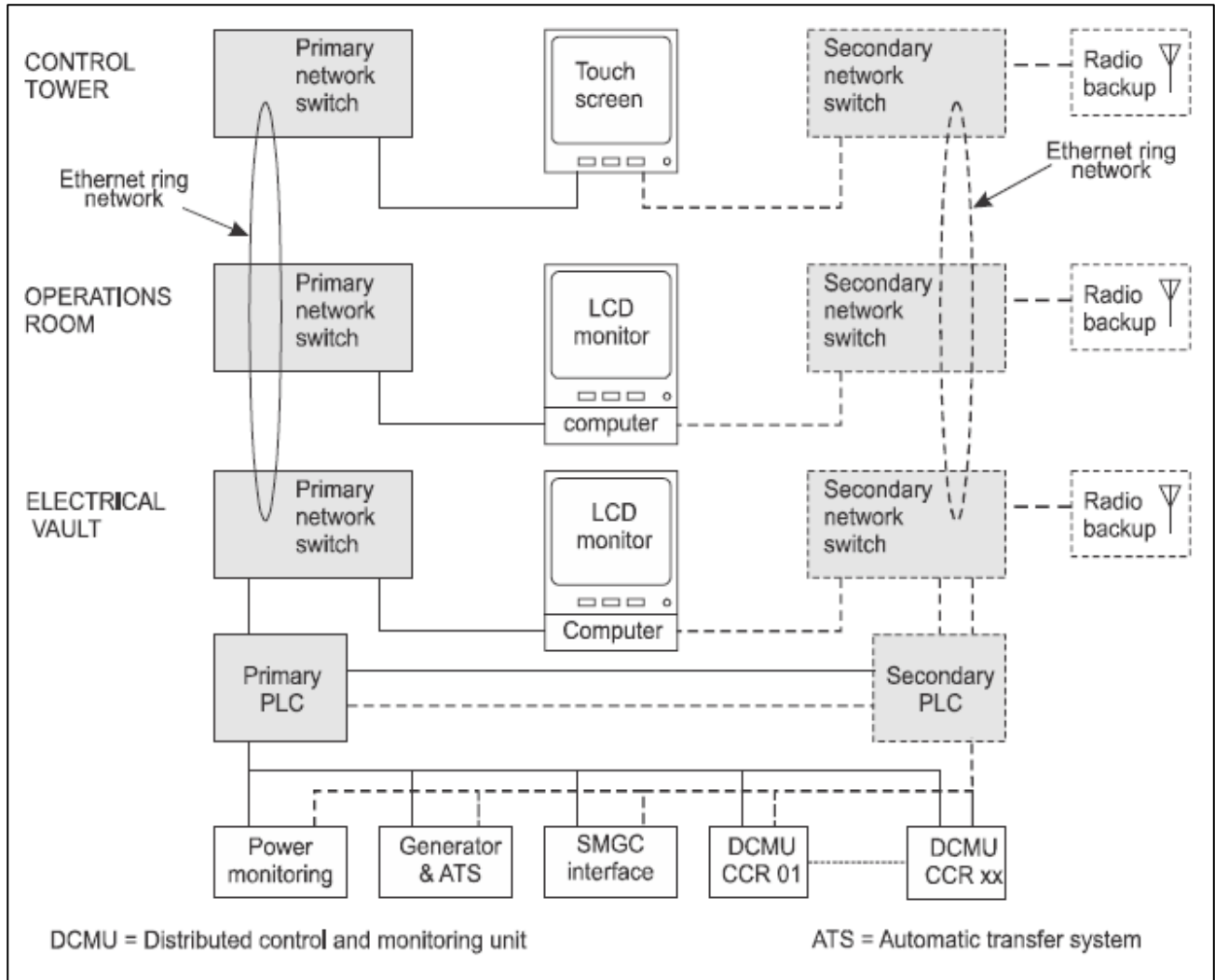
Figure 9-4. Aerodrome lighting computer system (ALCS)
