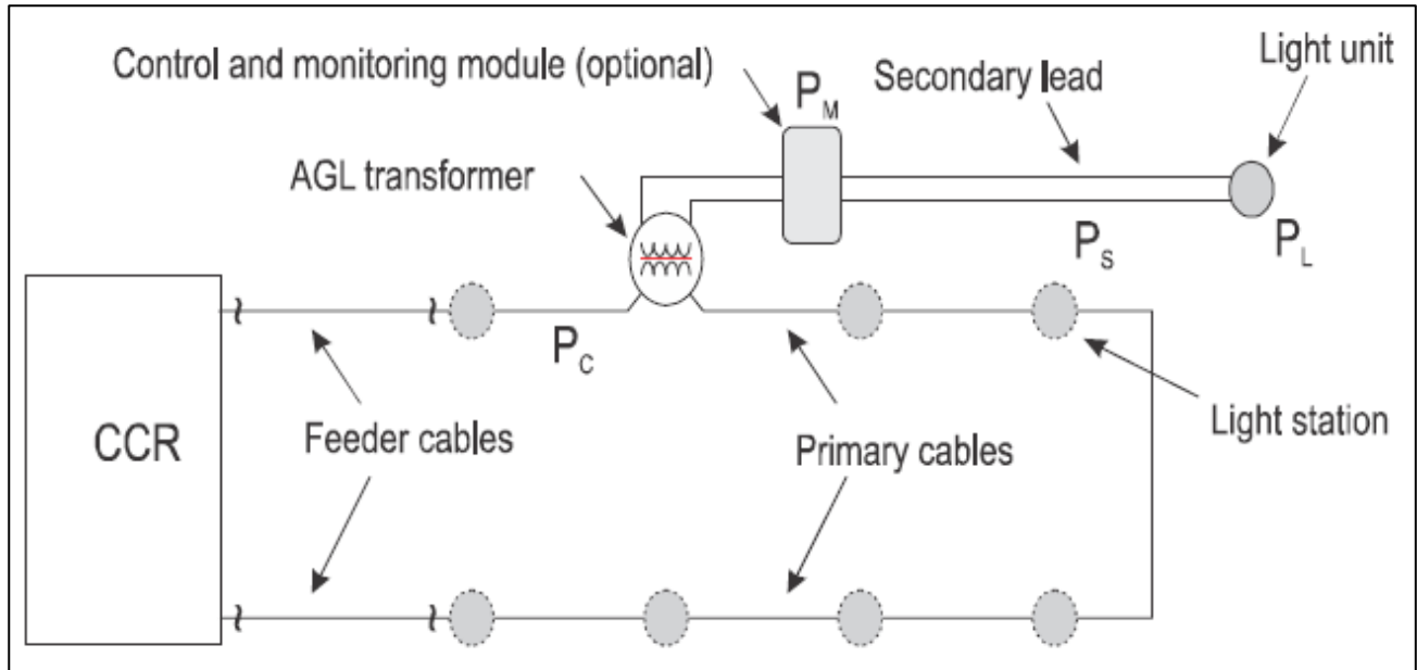
Figure 7-1. Circuit loading
