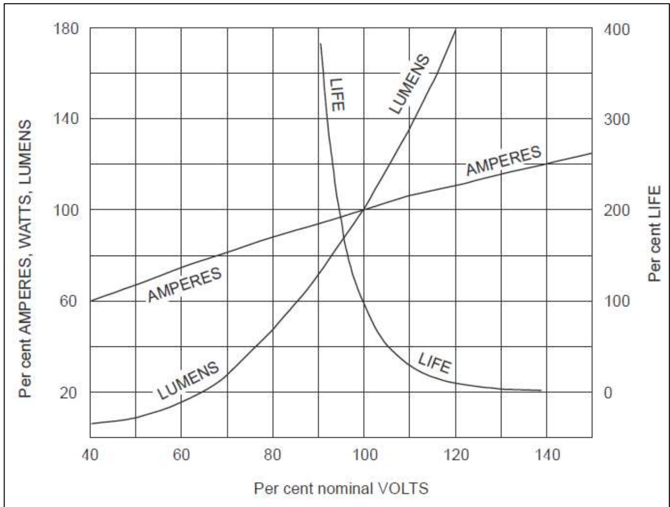
Figure 10-1. Effect of voltage variation on the operating characteristics of incandescent filament lamps in general lighting (multiple) circuit (adapted from IES Lighting Handbook 1984)
