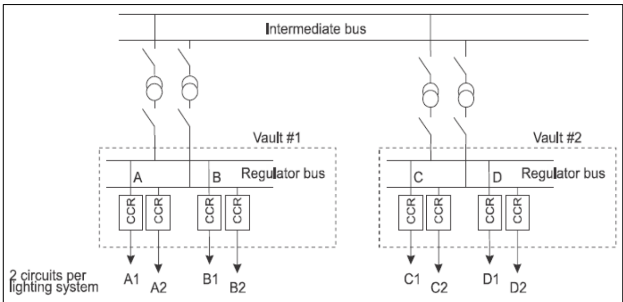
Figure 5-1. Provision of interleaved circuits
