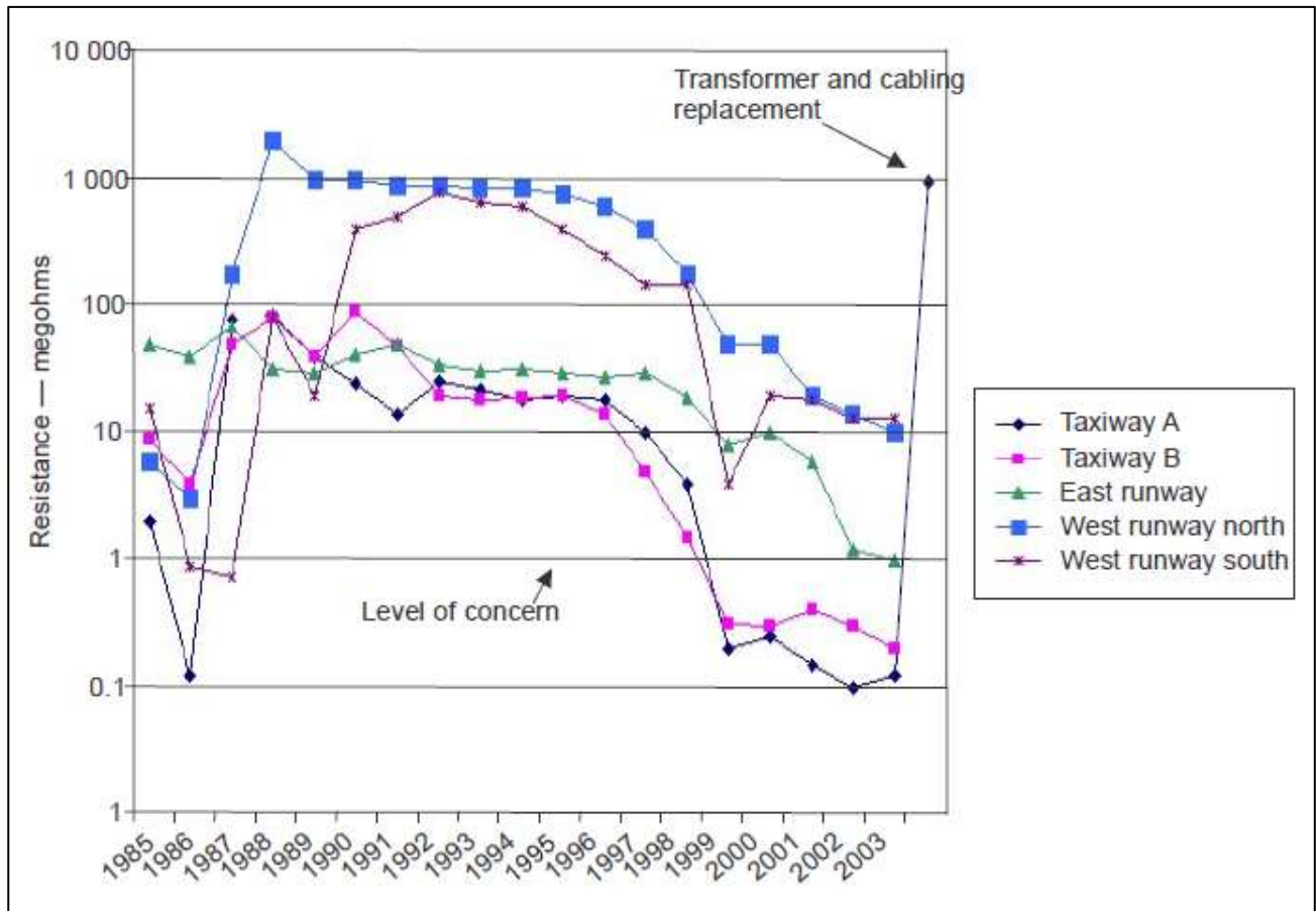
Figure 16-2. Example of insulation resistance measurements
