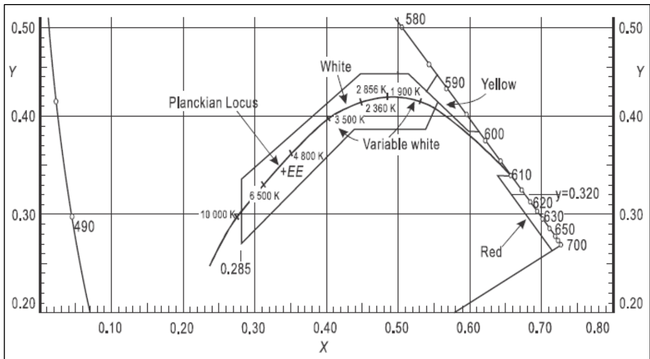
Figure 11-2. White and variable white for incandescent lighting
