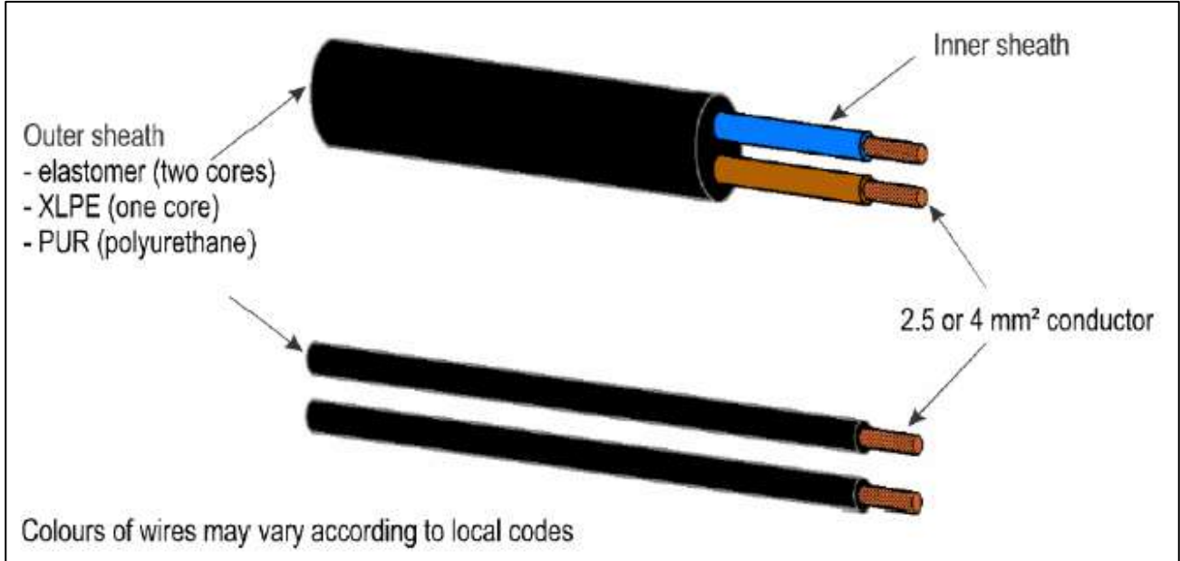
Figure 13-1. Secondary wire
