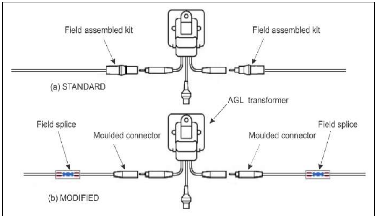
Figure 13-7. Primary connections with field splices
