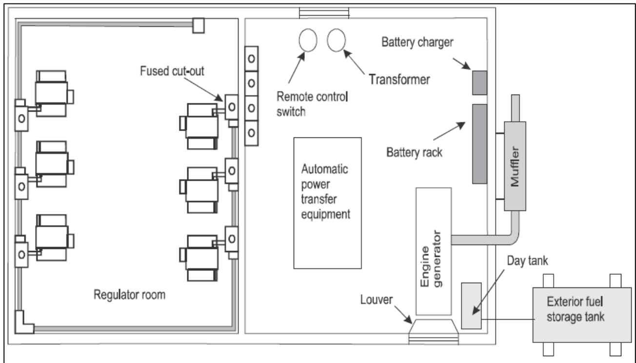
Figure 2-9. Electrical vault (source: UFC-3-535-01)
