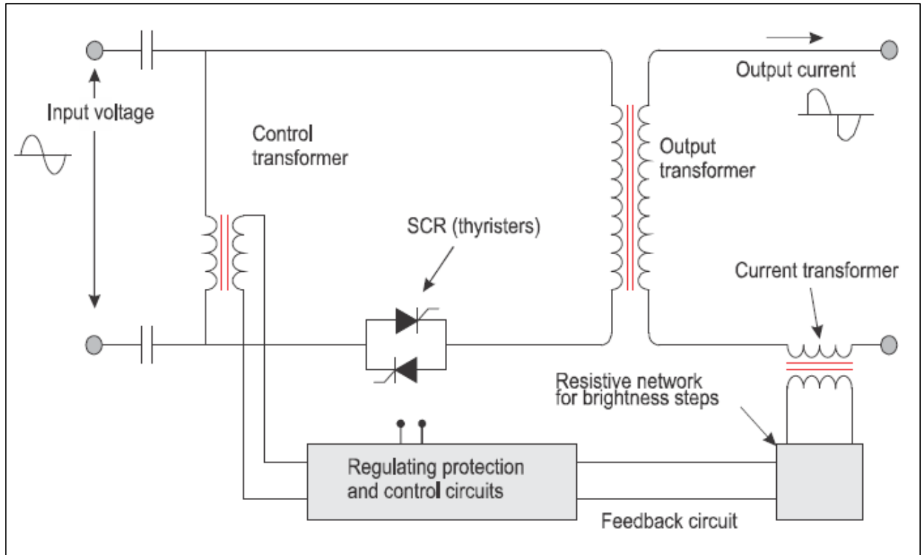
Figure 6-4. Solid state (SCR) regulator
