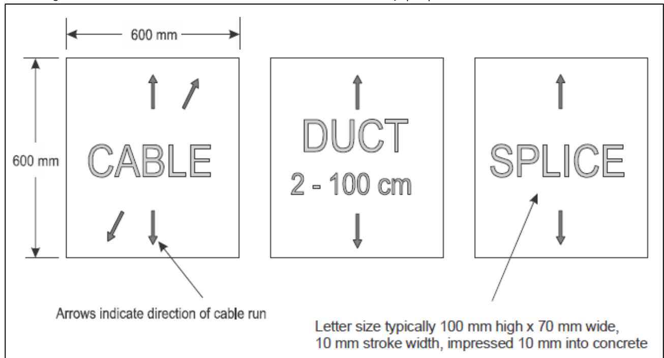
Figure 12-18. Cable markers
