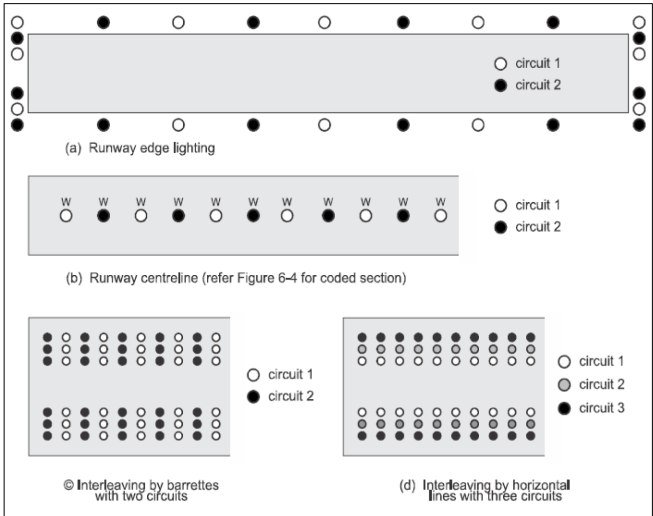
Figure 5-5. Runway edge, centreline and touchdown zone lighting
