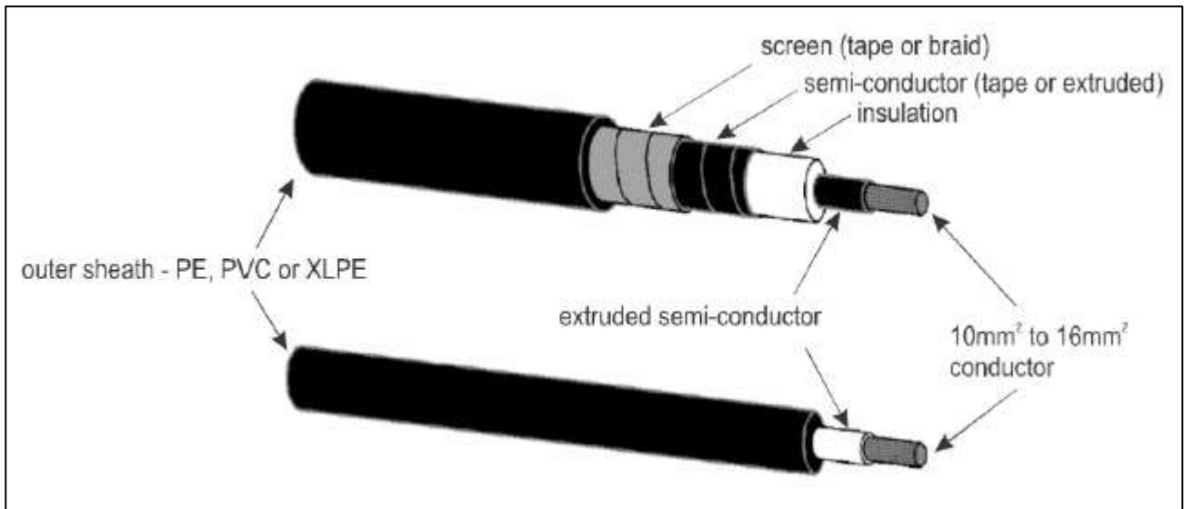
Figure 13-2. Primary cable
