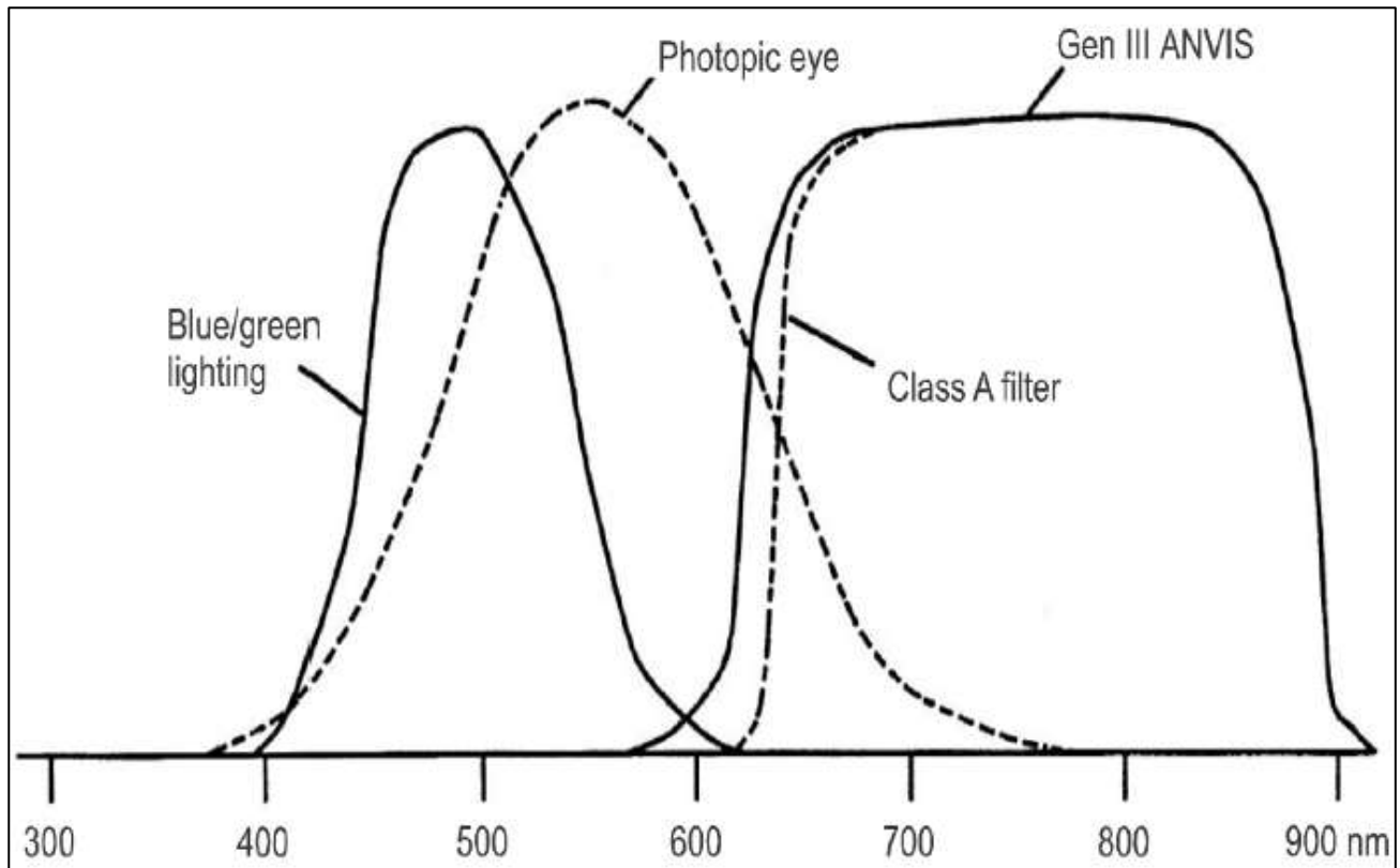
Figure 11-15. Class A filter allows blue/green cockpit lighting (source: Dennis L. Schmickley, Boeing Helicopter Co.)
