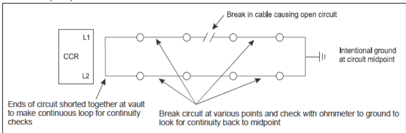
Figure 15-5. Locating open circuit faults
