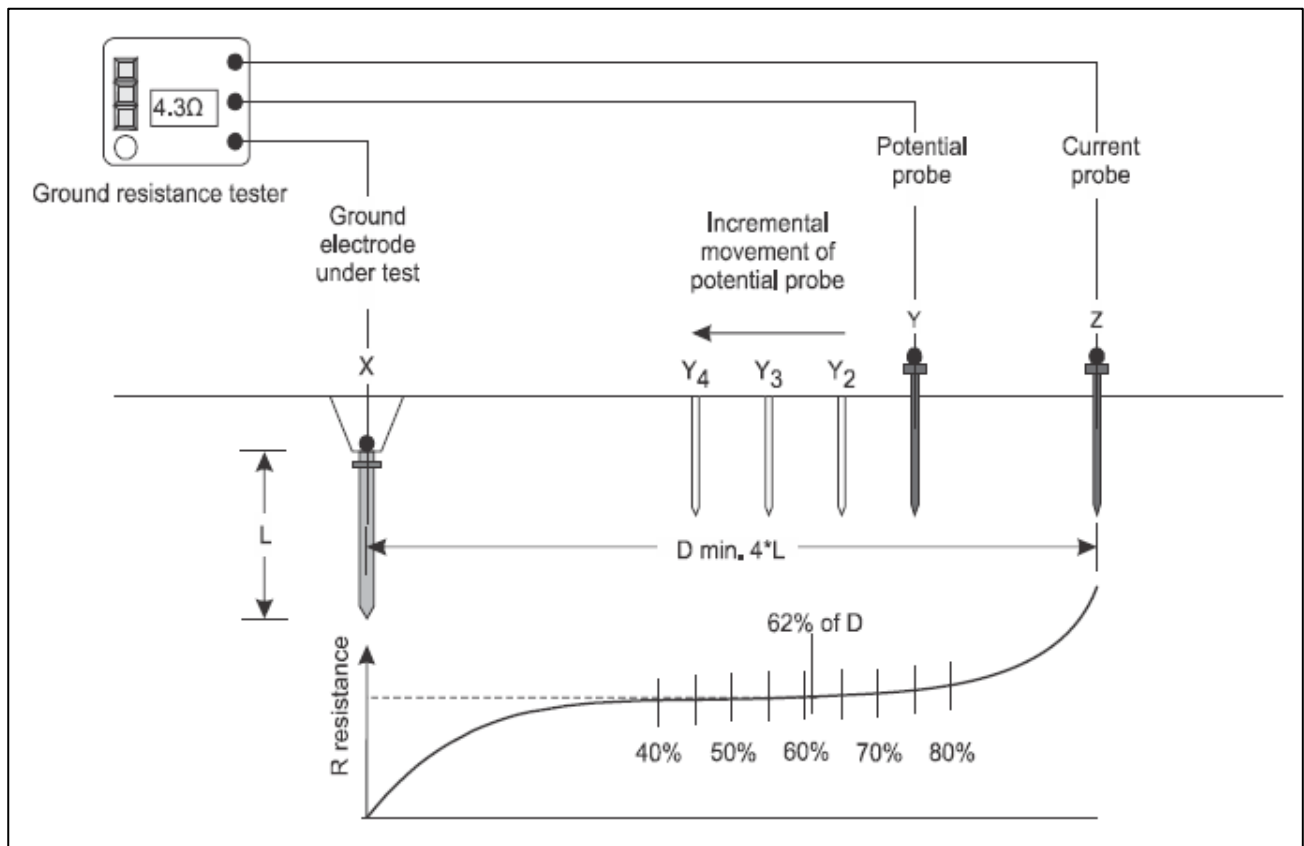
Figure 16-3. Ground resistance testing
