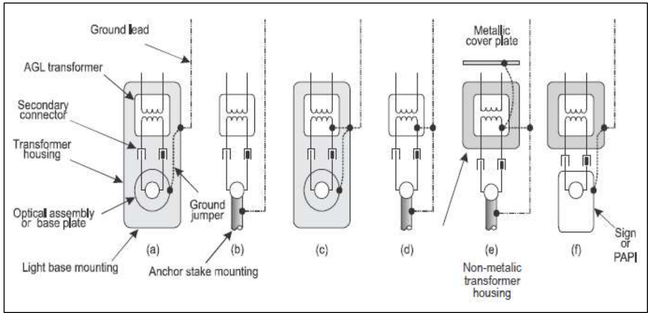
Figure 12-2. Light station equipment installation
