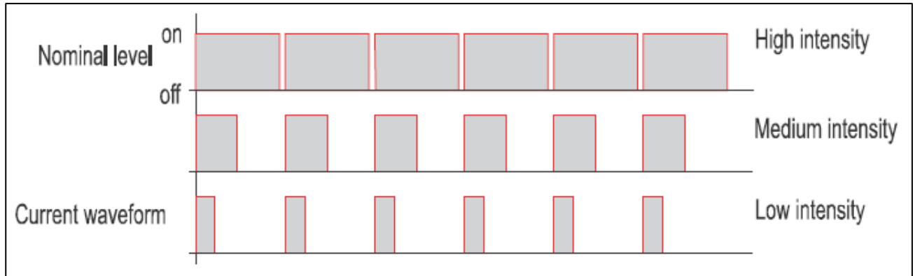
Figure 11-5. Intensity control by PWM
