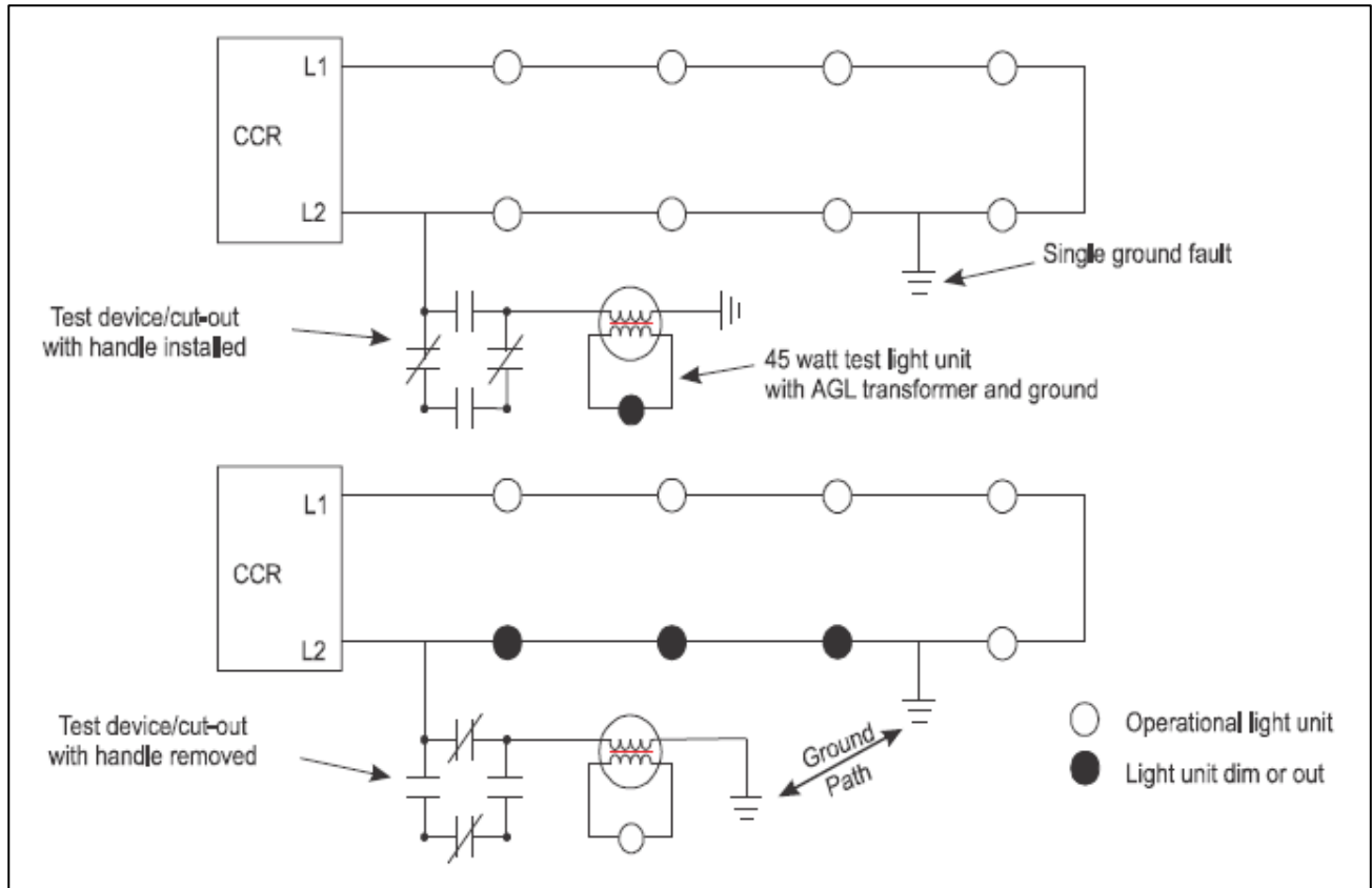
Figure 15-9. Intentional ground preventive maintenance tool
