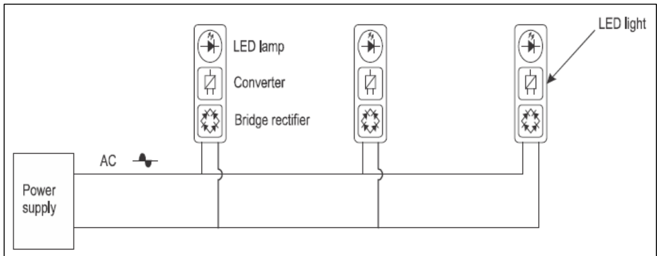
Figure 11-6. Parallel circuit for LED lighting
