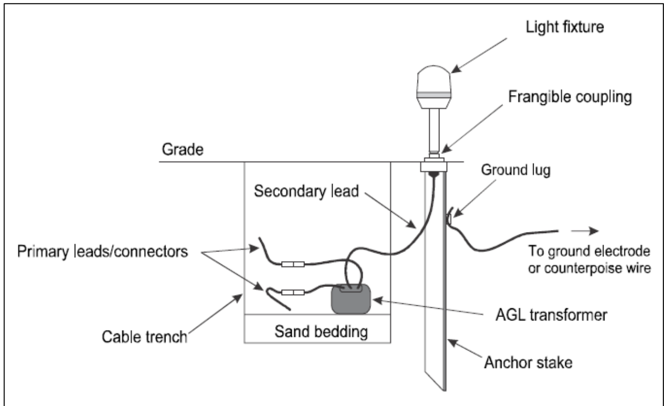
Figure 12-19. Direct burial of AGL transformer with stake-mounted light fixture
