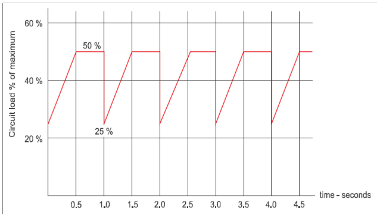
Figure 7-2. RGL load characteristic
