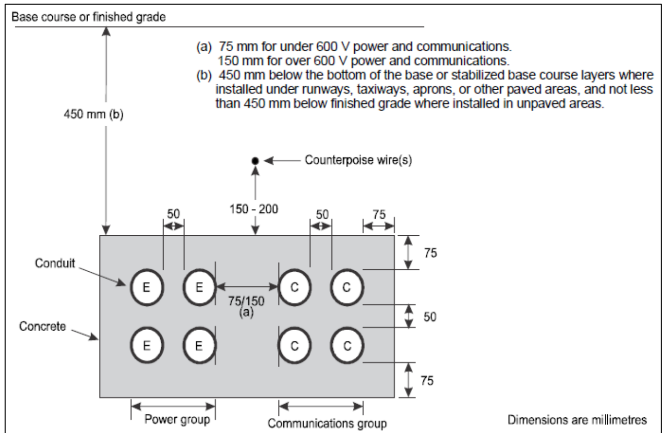
Figure 12-11. Concrete encased duct bank
