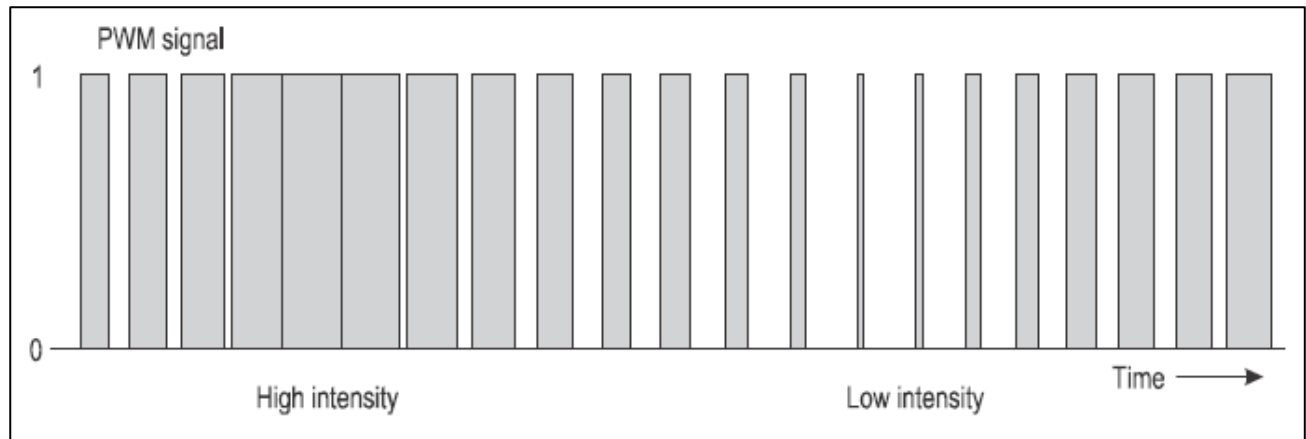
Figure 6-6. Delta modulation to generate PWM signal
