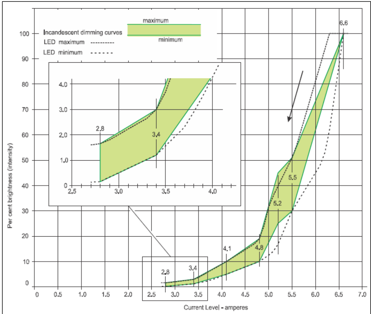
Figure 11-11. Dimming curves, coloured light
