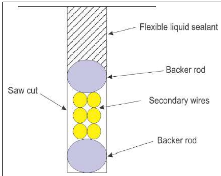
Figure 12-16. Secondary wireway saw cut for in-pavement lights
