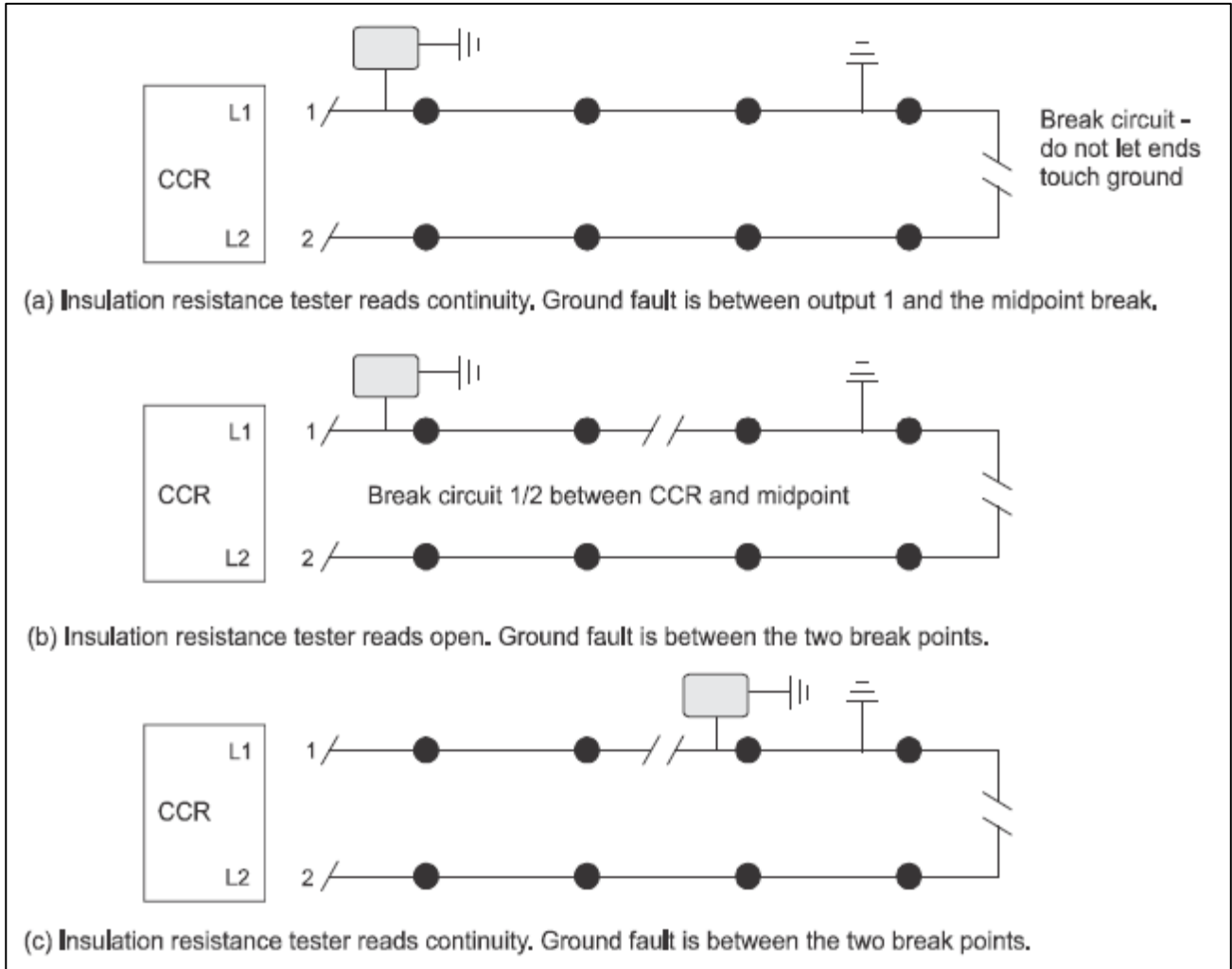
Figure 15-4. Alternative method using VOM or insulation resistance tester
