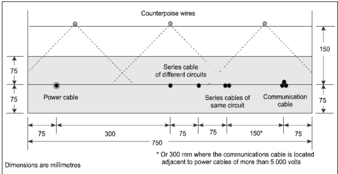
Figure 12-6. Installation in rock area
