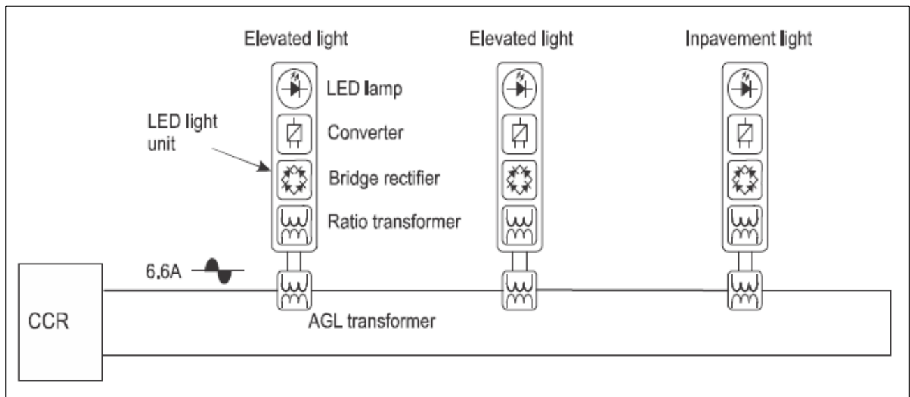
Figure 11-4. Series circuit LED lighting
