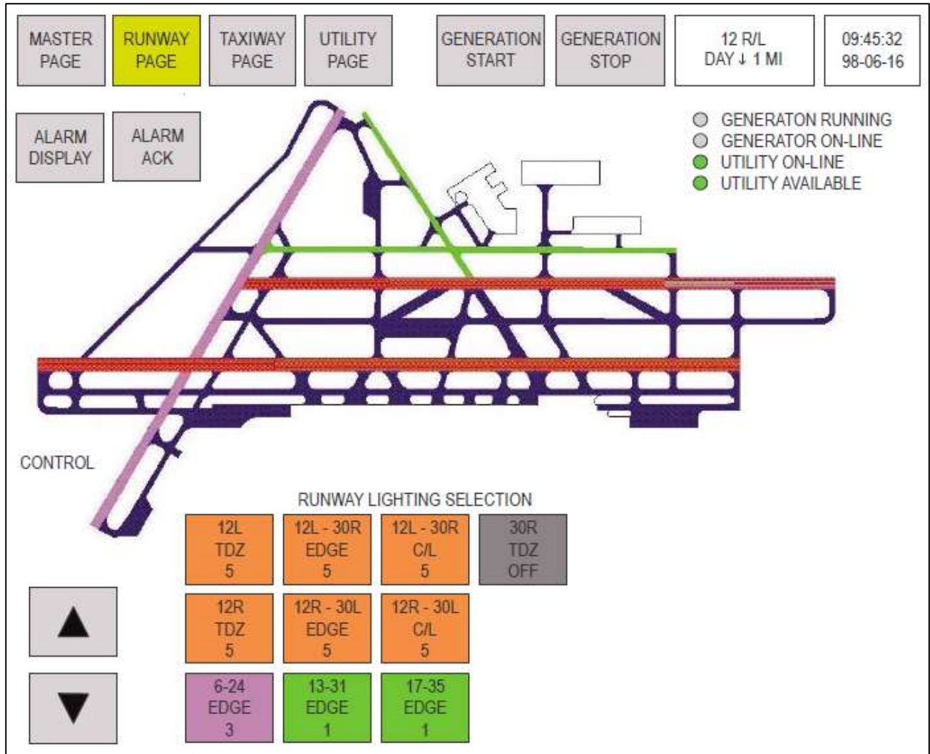
Figure 9-6. Mimic diagram and buttons on touch-sensitive screen (source: ADB Airfield Solutions)
