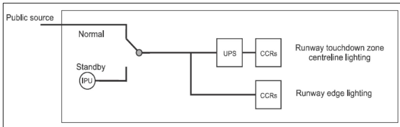
Figure 2-5. Separation of lighting facilities
