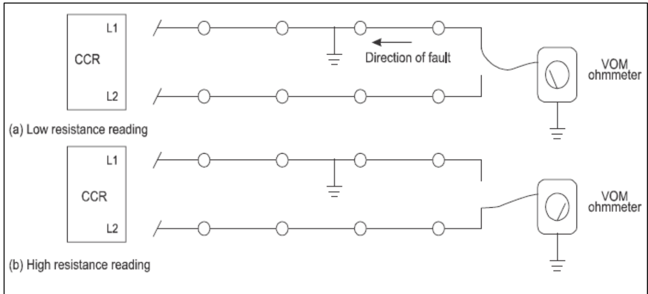
Figure 15-3. Locating ground faults with the VOM
