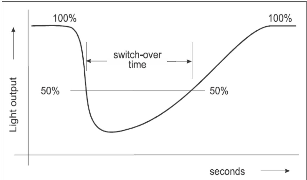
Figure 2-6. Transfer (switch over) time characteristic
