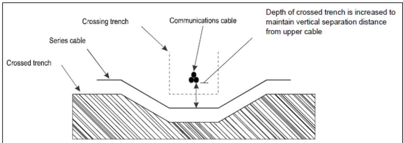
Figure 12-8. Crossover of cables
