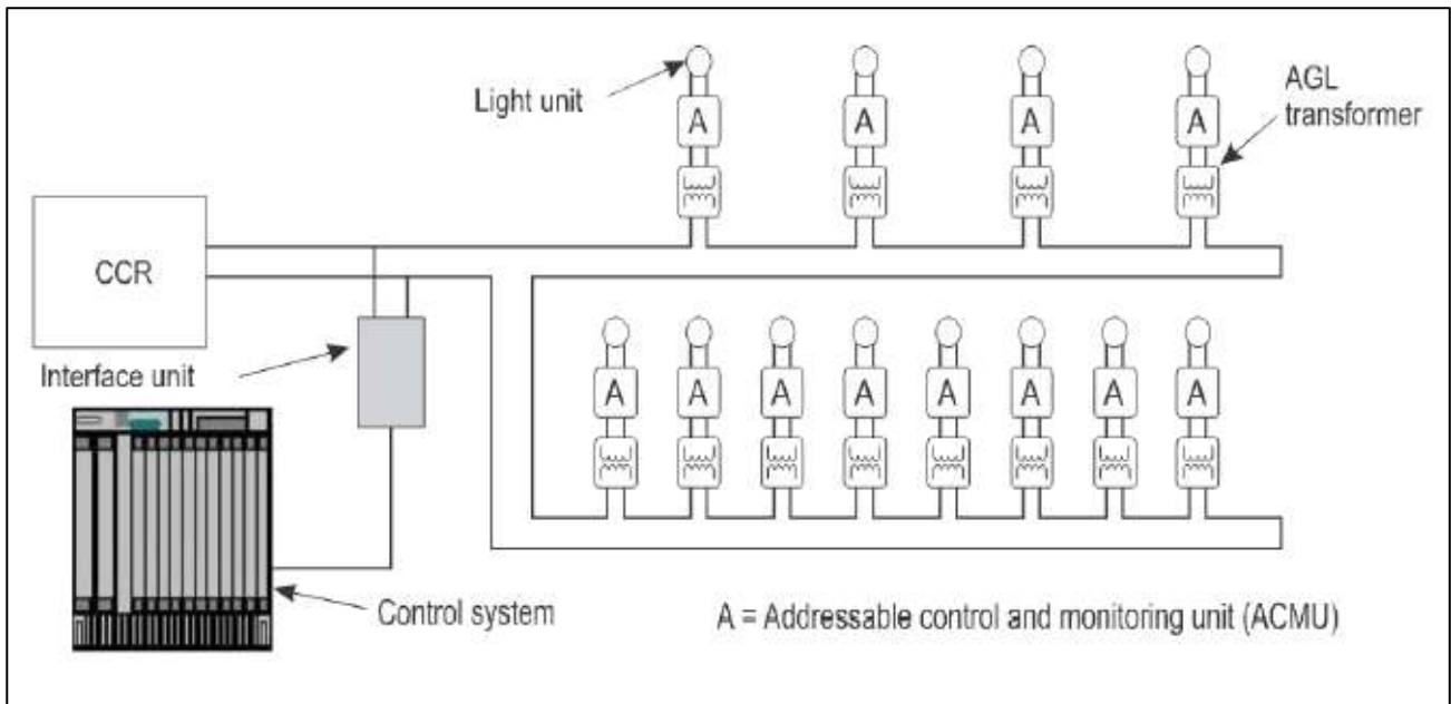
Figure 9-10. Addressable lights
