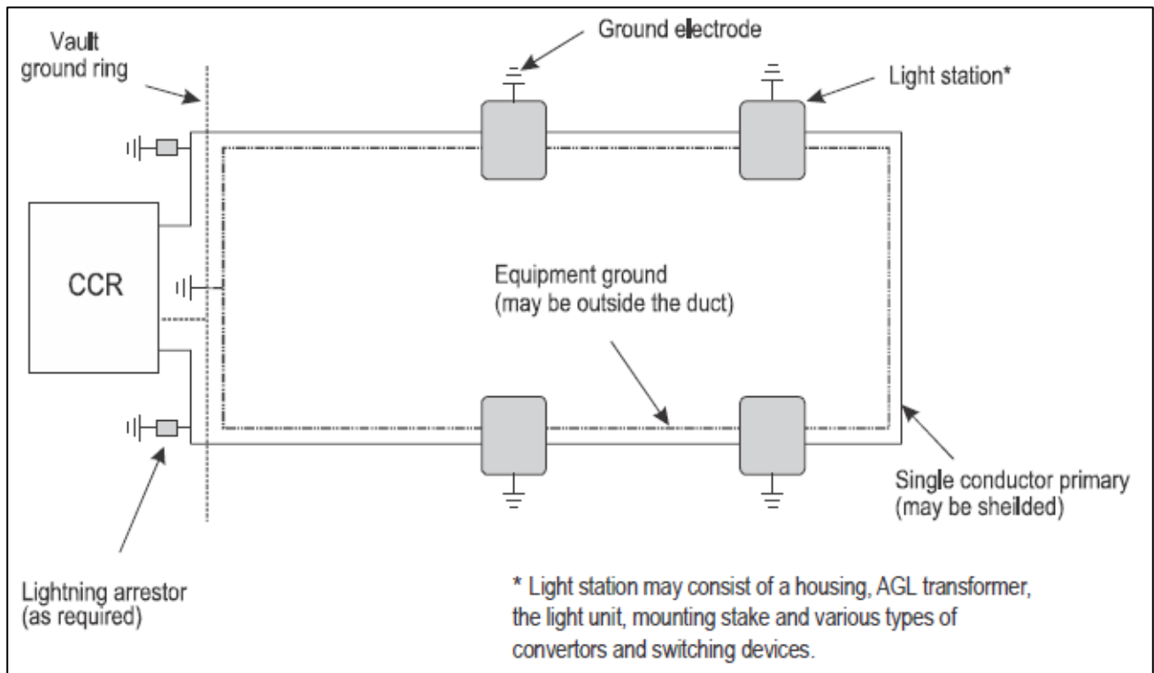
Figure 12-1. Typical constant current series circuit
