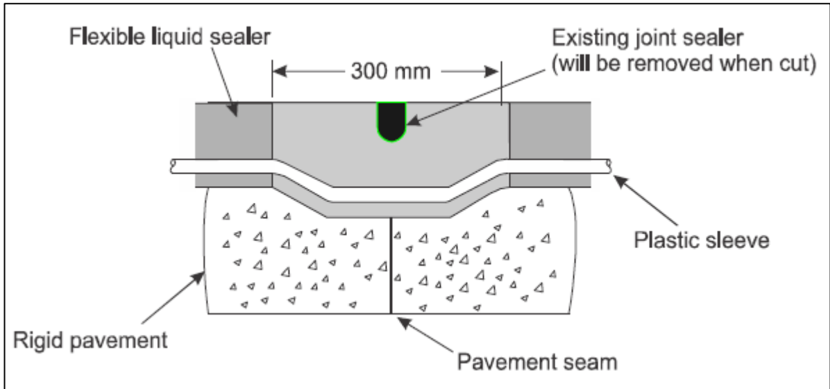
Figure 12-15. Joint crossing
