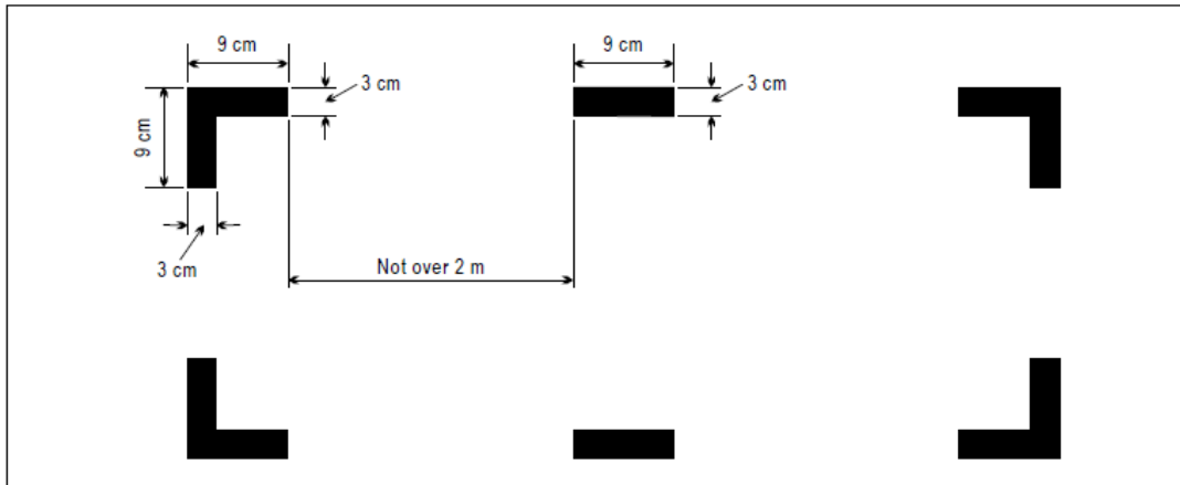
Figure 11 MARKING OF BREAK-IN POINTS (see 2.4)
