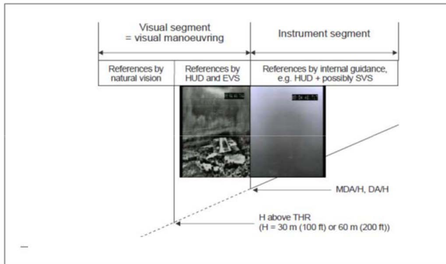
Figure 16 H-1. EVS Operations - Transition from Instrument to Visual
