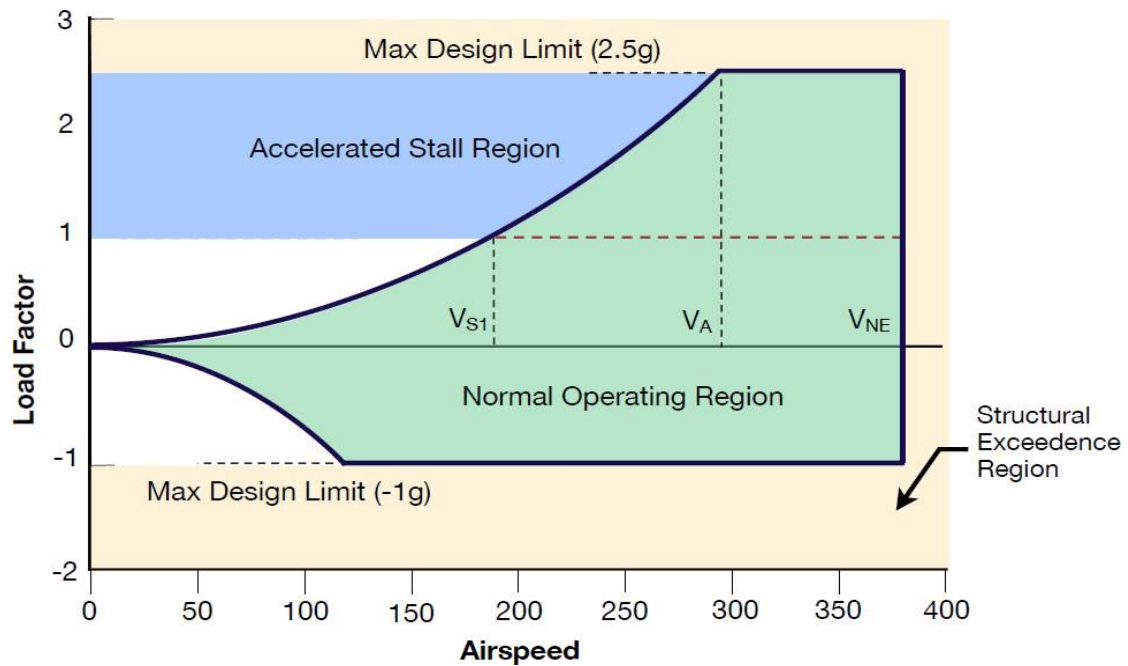
Figure 1 — V-n diagram (example)
