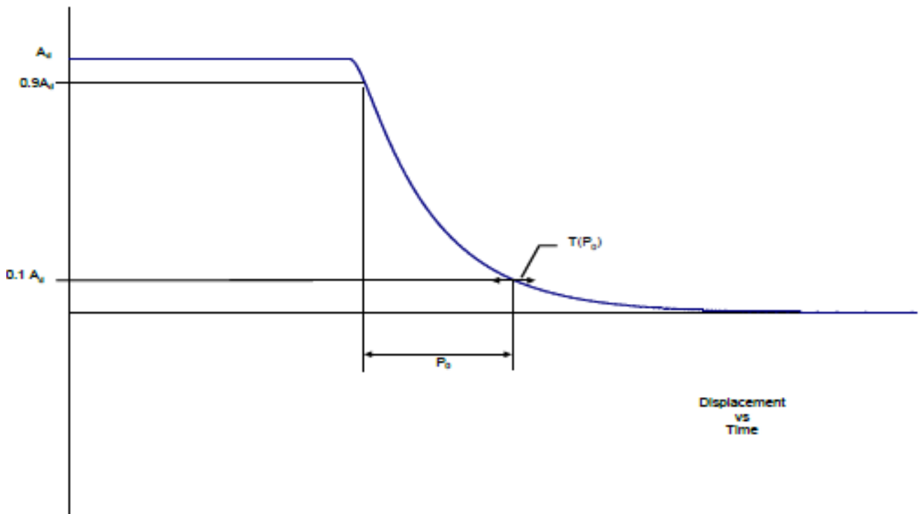
Figure 2: Critically damped step response
