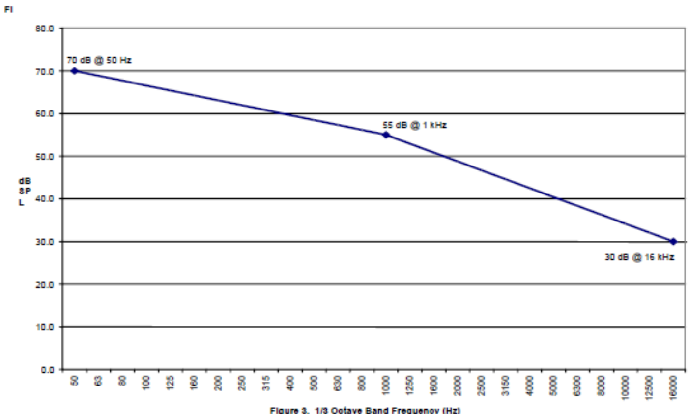
Figure 3: 1/3 octave band frequency (Hz)
