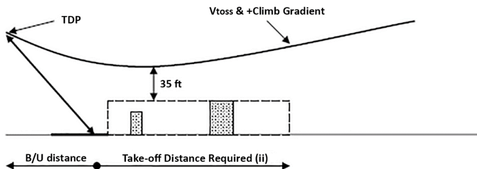
Figure 3 Helipad take-off
