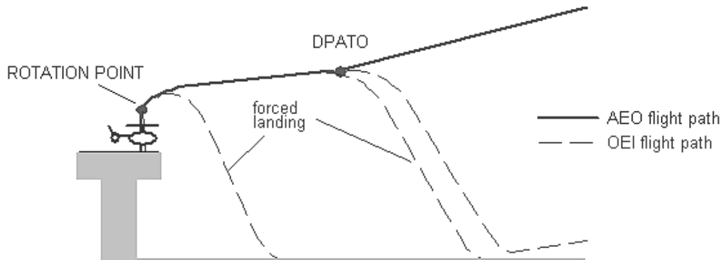
Figure 1 Take-off profile
